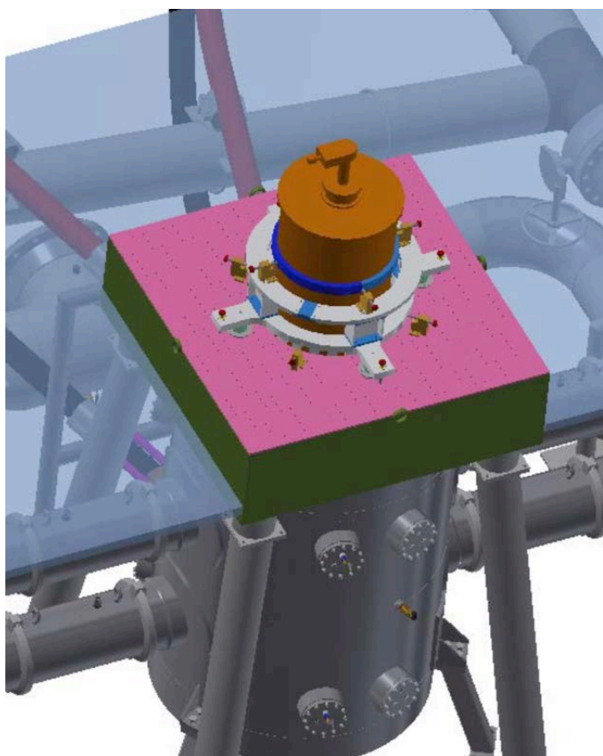
Figure 7: 41T cryostat vibration isolation platform.
