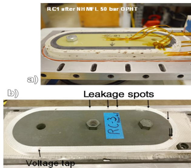
Figure 15: Alumino-silicate braided racetrack coils RC-1 (a) and RC-3 (b). A clear difference can be seen in the amount of leakage between RC-1 without and RC-3 with the TiO_2 coating.
