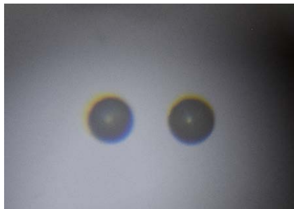
Figure 9 (a) A camera, a laser level (at the foreground) and a periscope (at the background) mounted at the hybrid platform. (b) The periscope and other parts of the optical setup mounted near the hybrid. (c) An image obtained by the setup described in text: two 1/16" balls located in the hybrid bore at ~11.5 T.
