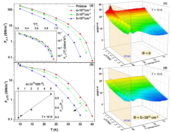
Figure 22: (a)-(b) Analysis of the pinning force density in a NdFeAs(O,F) thin film before and after irradiation with \alpha -particles: (a) interface (or “surface”) contribution F_{p,S} , (b) point defect contribution F_{p,PD} . The inset of (a) shows F_{p,S} normalized to T_c^2 ; the inset of (b) shows that F_{p,PD}/F_{p,S} is proportional to the fluence (c)-(d) n -value (as determined by the I - V characteristics) as a function of magnetic field and angle with the ab -planes for the same film before (c)
