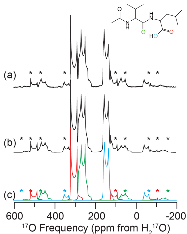
Figure 2. Experimental ^{17}\text{O} MAS NMR of N-Ac-VL (a), full simulation of MAS NMR spectrum (b) and simulation of each individual oxygen environment (c) at 21.1 T ( \omega_{\text{OH}}/2\pi = 900 MHz). Line structure is shown in the inset indicating the ^{17}\text{O} enriched sites: CO (red), NCO (green) and COH (blue). Spectra were acquired with \omega_{\text{R}}/2\pi = 24 kHz, spinning sidebands are noted by asterisks (*). NMR parameters used in spectral simulations are given in Table 4.
