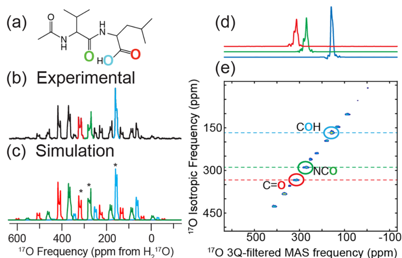
Figure 3. 1D and 2D ^{17}\text{O} MAS NMR spectra of [\text{U-}^{13}\text{C}, ^{15}\text{N}, 70\% ^{17}\text{O}] -N-Ac-VL recorded at 35.2 T ( \omega_{\text{OH}}/2\pi = 1500 MHz). Line structure (a) of N-Ac-VL illustrating the positions labeled with ^{17}\text{O} (NCO, CO, and COH). Experimental (b) and simulated (c) 1D MAS ^{17}\text{O} MAS NMR spectra, spinning at 19 kHz; centerbands indicated with asterisks (*). Slices (d) of the anisotropic dimension of the 2D 3QMAS spectrum of N-Ac-VL extracted at the isotropic frequency of the centerbands of each ^{17}\text{O} moiety. (e) 2D 3QMAS spectrum of [\text{U-}^{13}\text{C}, ^{15}\text{N}, 70\% ^{17}\text{O}] -N-Ac-VL at 35.2 T ( \omega_{\text{OH}}/2\pi = 1500 MHz) with the centerbands indicated with dashed horizontal lines and circles, the remaining peaks in the spectrum are due to spinning sidebands.
