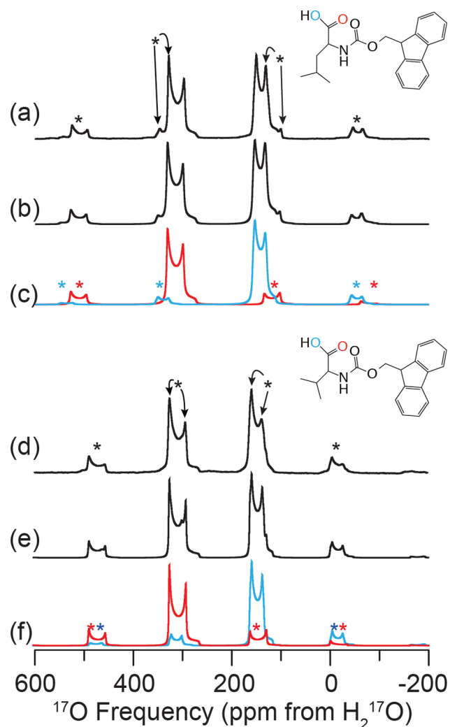
Figure 1. Experimental and simulated ^{17}\text{O} MAS NMR of Fmoc-L-leucine (a–c) and Fmoc-L-valine (d–f) at 21.1 T ( \omega_{\text{OH}}/2\pi = 900 MHz). Experimental ^{17}\text{O} MAS NMR (a,d), full spectral simulations (b,e), and simulations of each individual oxygen environment, CO (red) and COH (blue) (c,f) are shown. The line structures of Fmoc-L-leucine (inset above (a)) and Fmoc-L-valine (inset above (d)) indicating the oxygen environments of interest are displayed. Spectra were acquired with \omega_{\text{R}}/2\pi = 24 (Fmoc-L-leucine) or 20 (Fmoc-L-valine) kHz, with spinning sidebands noted by asterisks (*). NMR parameters used in spectral simulations are given in Table 4.
