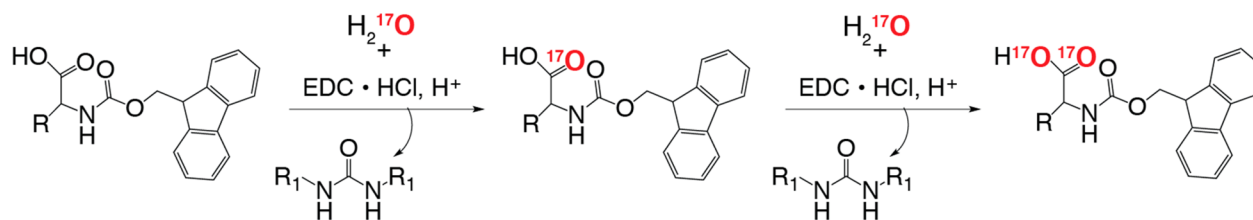
Scheme 1. Isotopic Labeling of Fmoc Amino Acids Using the Multiple-Turnover Reaction with 1-Ethyl-3-(3-dimethylaminopropyl)carbodiimide Hydrochloride (EDC·HCl) 59
