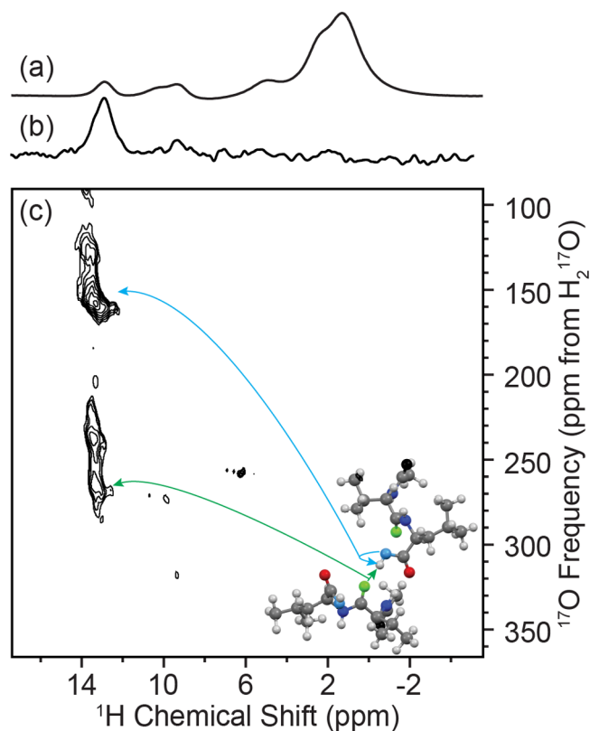
Figure 7. MAS NMR spectroscopy of N-Ac-VL: (a) 1 H direct Hahn-echo detection, (b) one-dimensional 1 H– 17 O R 3 -R-INEPT, (c) and two-dimensional 1 H– 17 O R 3 -R-INEPT spectrum with R 3 = 100 μs. Spectra were acquired with ω R /2π = 20 kHz at 17.6 T (ω OH /2π = 750 MHz). Correlations between the leucine carbonyl proton to its directly bonded oxygen (blue arrow) and its next closest oxygen through space (NCO, green arrow) are indicated on the crystal structure of N-Ac-VL in the inset. 92
