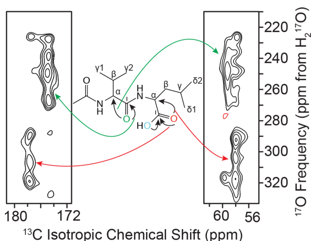
Figure 6. Two-dimensional ^{13}\text{C} – ^{17}\text{O} ZF-TEDOR spectrum recorded at 21.1 T ( \omega_{\text{OH}}/2\pi = 900 MHz) with 2.4 ms of mixing. Correlations between the NCO and CO oxygen sites with the closest \text{C}' and \text{C}\alpha indicated on the line structure of N-Ac-VL in the inset.
