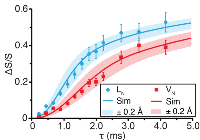
Figure 4. One-dimensional 15 N– 17 O REAPDOR dephasing curves of the leucine (blue, circle) and valine (red, squares) nitrogens of N-Ac-VL at 17.6 T ( \omega_{\text{OH}}/2\pi = 750 MHz). Best-fit simulated REAPDOR dephasing curves (solid lines) and \pm 0.2 Å error (semi-transparent curve) in simulated dephasing curves generated using SIMPSON. 76 15 N– 17 O distances that were determined based on the simulated curves are given in Table 5.
