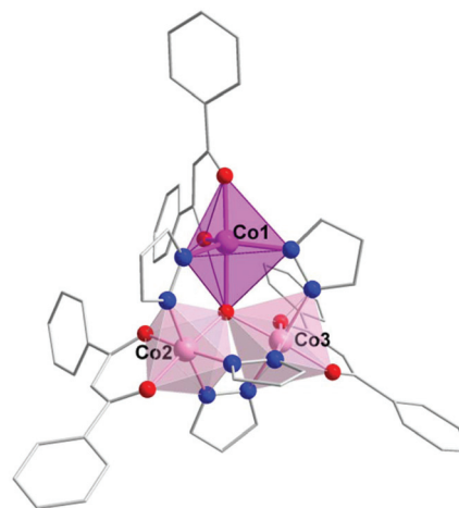
Fig. 1 The molecular structure of 1 . Colour code: Co II : dark pink (the dark pink polyhedron represents the TBP geometry), Co III : light pink (the light pink polyhedra represent the octahedral geometry), O: red, N: blue, C: grey. Hydrogen atoms are omitted for clarity.
