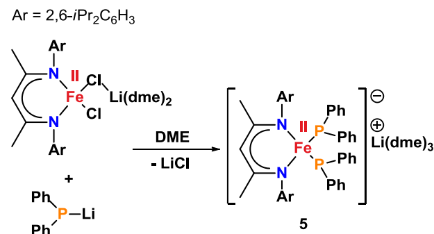
Scheme 3. Synthesis of complex 5 .
