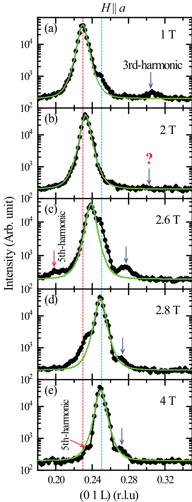
FIG. 3. L-scans measured along (0\ 1\ L) at selected fields, T = 1.5\ \text{K} . (a) \mu_0 H = 1\ \text{T} ; (b) \mu_0 H = 2\ \text{T} ; (c) \mu_0 H = 2.6\ \text{T} ; (d) \mu_0 H = 2.8\ \text{T} ; (e) \mu_0 H = 4\ \text{T} . The intensity is plotted in logarithmic scale. The blue and red arrows point to the third-order
