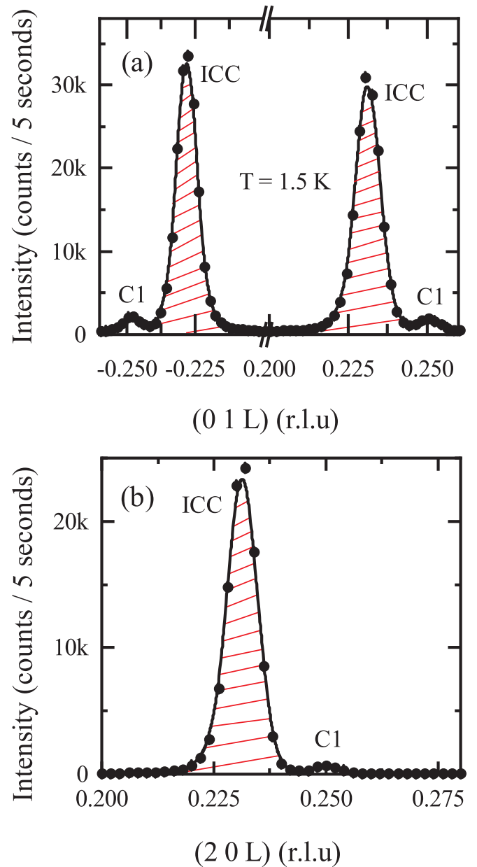
FIG. 1. L-scans along (a) (0\ 1\ L) and (b) (2\ 0\ L) directions illustrate the coexistence of incommensurate (ICC, wave vector k_1 = (0\ 0\ k_{z1}) , k_{z1} \approx 0.23 ) and commensurate (C1, wave vector k_2 = (0\ 0\ k_{z2}) , k_{z2} \approx 0.25 ) phases at 1.5 K and 0 T.
