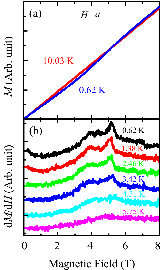
FIG. 4. Magnetization (a) and the first derivative of the magnetization (b) measured with H \parallel a . Two peaks are observed in dM/dH corresponding to the complete suppression of the ICC phase and the spin-flop transition.
