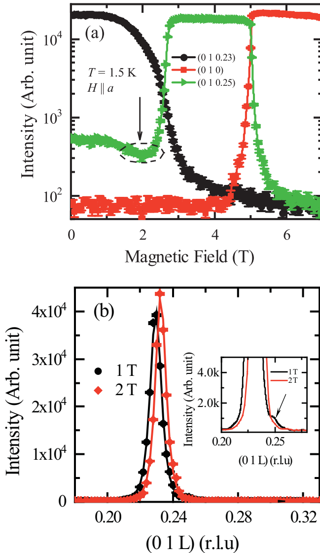
FIG. 2. Neutron diffraction data measured with H \parallel a at 1.5 K. (a) Neutron diffraction intensity as a function of magnetic field obtained by counting at the peak position of (0 1 0.23), (0 1 0.25), and (0 1 0) magnetic peaks. The (0 1 0.23), (0 1 0.25), and (0 1 0) peaks are associated with the incommensurate ICC, commensurate C1 and C2 states as described in the text. The black arrow and the ellipse in dashed line indicate an anomalous dip between 1.5 T and 2.5 T in the data of the (0 1 0.25) peak. (b) L-scans along (0 1 L) measured at \mu_0 H = 1 , and 2 T. The inset depicts the disappearance of the weak (0 1 0.25) peak at 2 T.
