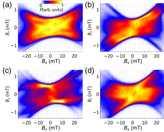
FIG. 5. (a)–(d) Intensity maps of the integrated magnetization noise P = \int S(\nu) d\nu versus in-plane and out-of-plane applied field ( B_x , B_z ), at room temperature (295 K). The four panels are acquired at slightly different locations on the Pt/Co/Pt film, separated by < 10 \mu\text{m} . The bow-tie shape of these images is determined by the balance between the fixed thermal energy k_B T and the field-dependent energy required to spontaneously form magnetic domains (see text). The very different patterns within each bow tie, and the lack of reflection symmetry about the B_{x,z} = 0 axes, reveal a spatially varying magnetic anisotropy that is canted slightly away from perfectly out of plane. Dashed line in (a) shows a quadratic fit to the edge of the bow tie.
