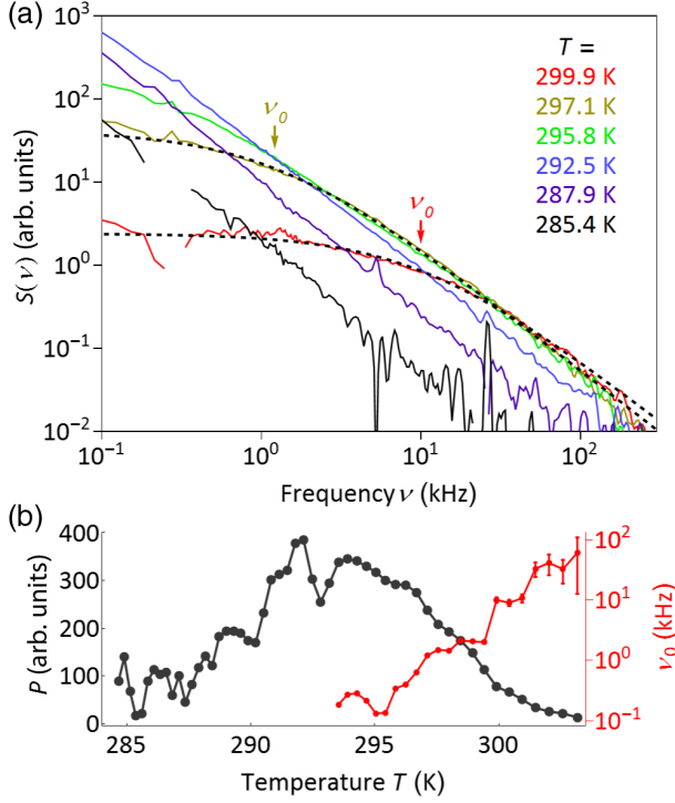
FIG. 3. (a) Magnetization noise spectra S(\nu) at different temperatures T , measured at a fixed location on the trilayer that exhibits perpendicular magnetization at low temperatures ( T < 290 K), and in-plane magnetization at high temperatures ( T > 300 K). S(\nu) exhibits robust \nu^{-3/2} power-law behavior at low T . With increasing T , S(\nu) grows in magnitude but then develops a steadily increasing critical frequency \nu_0 , below which the noise tends toward spectrally flat. Again, all spectra can be empirically fit by S(\nu) \propto (\nu + \nu_0)^{-3/2} (dashed lines). (b) Integrated noise power P and critical frequency \nu_0 versus T , indicating that the SRT region has been temperature tuned through the fixed location of the probe.
