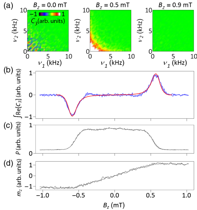
FIG. 7. Measuring higher-order correlations of the magnetization noise at a location on the sample near the SRT that exhibits linear magnetization and large fluctuations (similar to Fig. 4). (a) The real part of the third-order correlator, \text{Re}[C_3(\nu_1, \nu_2)] , acquired at B_z = 0, 0.5, and 0.9 mT. (b) The integral \int \text{Re}[C_3] d\nu_1 d\nu_2 measured as a continuous function of B_z . The red line shows this dependence calculated from the magnetic free energy (see Supplemental Material [35] for details). (c) The simultaneously measured total noise power P = \int S(\nu) d\nu versus B_z [similar to Fig. 4(c)]. (d) The average magnetization m_z(B_z) at this same location, as measured by conventional MOKE, showing a constant susceptibility for |B_z| < B_{\text{sat}} [similar to Fig. 4(a)]. The third-order correlator is approximately zero except when |B_z| \simeq B_{\text{sat}} , indicating a skewness in the distribution of \delta m_z(t) .
