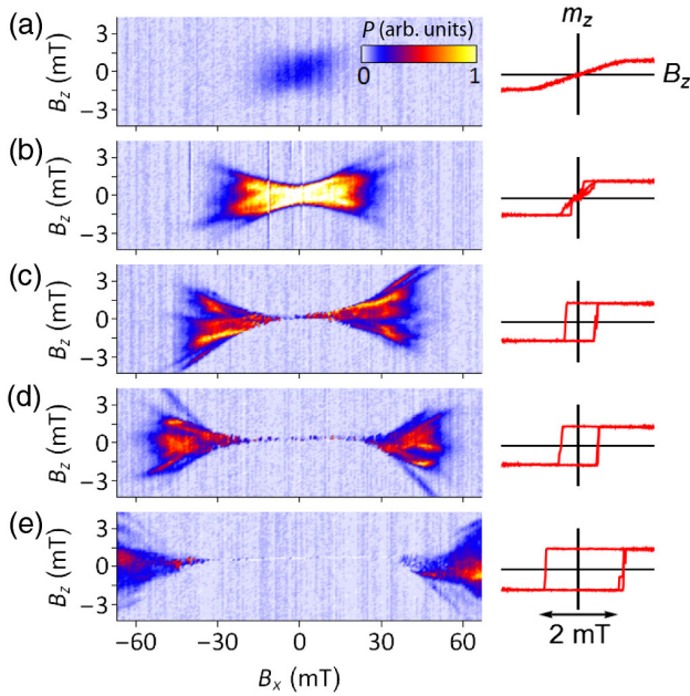
FIG. 6. Intensity maps of the integrated magnetization noise P(B_x, B_z) at different locations across the Pt/Co/Pt sample, beginning in (a) regions of the sample with in-plane magnetization, where P is small. (b) Near the SRT, P is large when |B_z| < B_{\text{sat}} (cf. Fig. 5). (c)–(e) In regions with less disorder and therefore increasingly stable perpendicular magnetization, \mu_0 H_c increases and fluctuations vanish at B_{x,z} = 0 . However, strong fluctuations reemerge when larger |B_x| is applied. Note that the m_z(B_z) magnetization curves are all acquired at B_x = 0 using a rapidly varying B_z (several Hz). This gives an open hysteresis loop with large switching (coercive) fields in panels (c)–(e). In the corresponding noise maps, B_z was ramped much more slowly (mHz), so that the film switched at very small B_z .
