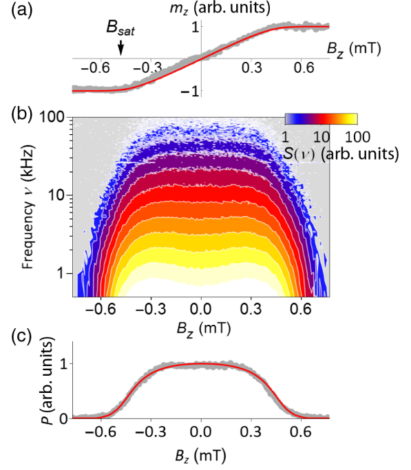
FIG. 4. (a) The average magnetization m_z versus applied perpendicular magnetic field B_z (measured by conventional MOKE), at a location on the trilayer near the SRT. m_z increases linearly with B_z (indicating constant magnetic susceptibility \chi = dm_z/dB_z ), until it saturates for |B_z| > B_{\text{sat}} . (b) Intensity map of the noise spectra S(\nu) at different B_z . For all |B_z| < B_{\text{sat}} , S(\nu) is unaffected (and follows \nu^{-3/2} ), but S(\nu) \rightarrow 0 when |B_z| > B_{\text{sat}} . (c) The integrated magnetization noise P = \int S(\nu) d\nu versus B_z . The correspondence between P and \chi is in accord with the fluctuation-dissipation theorem. Moreover, the detailed dependence of P (and m_z ) on B_z can be qualitatively captured by simple considerations of the free energy of a mixture of magnetic domains, as shown by the red lines in (c) and (a); see text.
