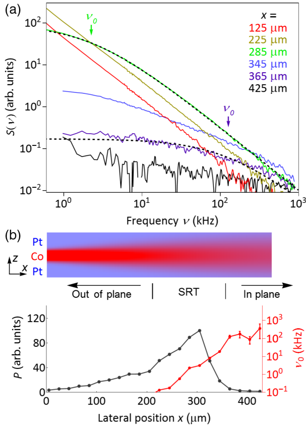
FIG. 2. (a) Power spectra of the magnetization fluctuations S(\nu) at different lateral positions x on the Pt/Co/Pt trilayer. In regions with perpendicular magnetization, S(\nu) \propto \nu^{-3/2} . Upon entering and traversing the SRT region, S(\nu) develops a steadily increasing critical frequency \nu_0 , below which the noise tends toward spectrally flat, consistent with an evolving low-frequency cutoff in the distribution of fluctuation rates. Empirically, all spectra can be fit by S(\nu) \propto (\nu + \nu_0)^{-3/2} (dashed lines). (b) The integrated noise power, P = \int S(\nu) d\nu , exhibits a peak in the SRT region. Concomitantly, \nu_0 rapidly increases through the measurement bandwidth (red points).
