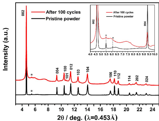
Fig. 7. SXR D patterns of a P2-Na 0.6 Li 0.2 Mn 0.8 O 2 electrode materials before and after long-term cycles, including an extended view of the impurity and superlattice region (inset).
