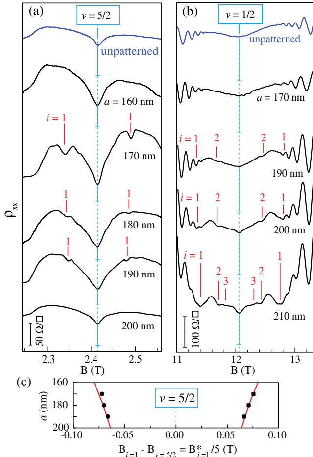
FIG. 2. Dependence of the GR features of CFs near (a) \nu = 5/2 and (b) \nu = 1/2 on the period of the surface superlattice. Magnetoresistance traces are vertically offset for clarity and the zero-resistance positions are indicated with blue horizontal marks. The expected positions for GRs are marked with red lines. (c) Summary of the positions of the observed GR minima (symbols) and expected values (lines) near \nu = 5/2 .
