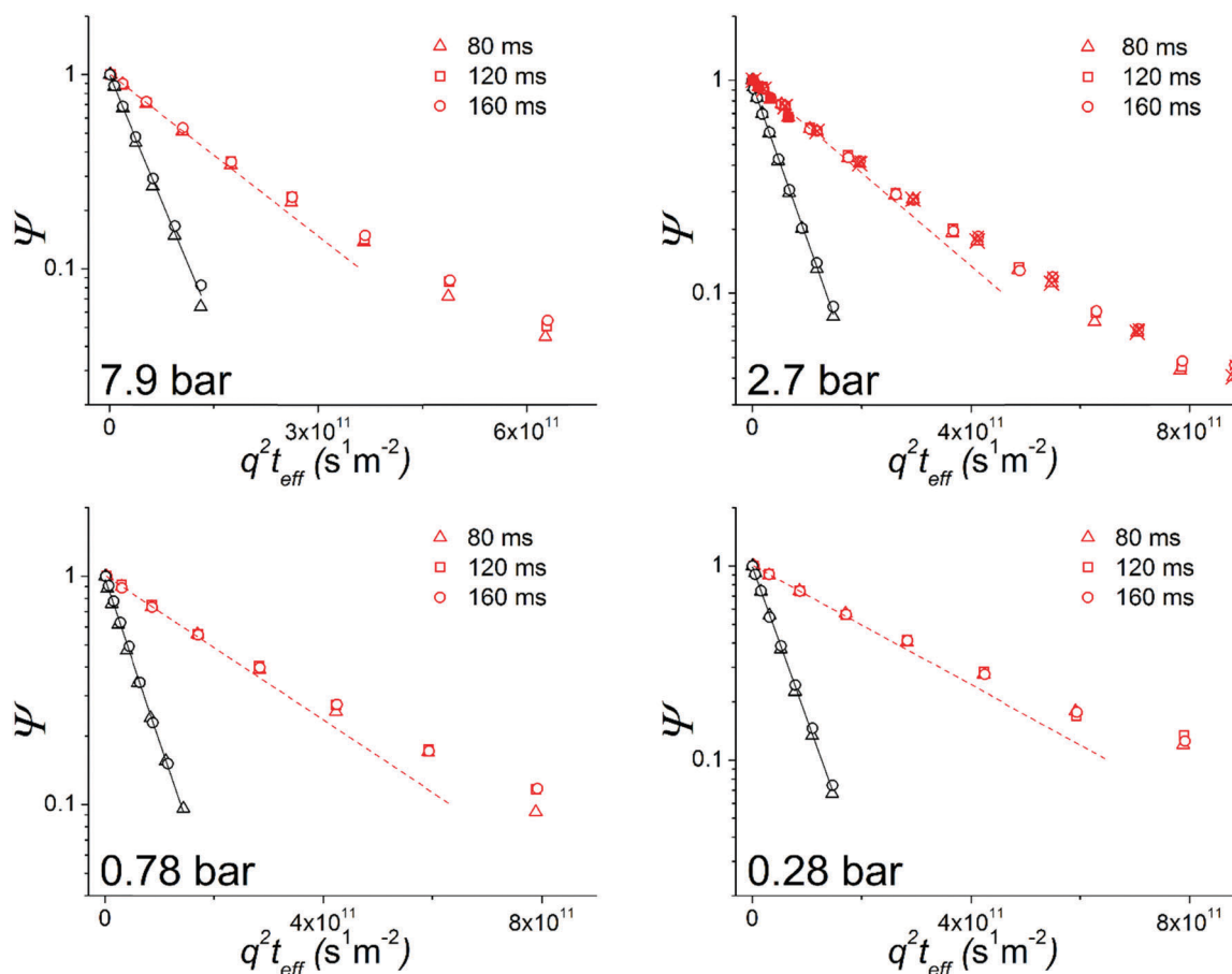
Fig. 1 ^{13}\text{C} PFG NMR attenuation curves for ethane diffusion in ZIF-7-8 (hollow red symbols) and ZIF-8 (hollow black symbols) at four different ethane loading pressures and at different diffusion times shown in the figure legends. Also shown for comparison is the initial part of the corresponding ^1\text{H} PFG NMR attenuation curve for ZIF-7-8 at the loading pressure of 2.7 bar (filled red triangles in the upper right figure). The solid black lines represent a monoexponential fit of the ZIF-8 data using eqn (1), while the dashed red line is the monoexponential fit using eqn (1) of the initial 30% of the signal attenuation in ZIF-7-8. Crossed symbols for the loading pressure of 2.7 bar correspond to the measurements at 17.6 T. Symbols without crosses correspond to the measurements at 14 T.
