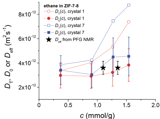
Fig. 5 Comparison of corrected diffusivities, D_0 , from IRM with the effective self-diffusivities, D_{\text{eff}} , from PFG NMR of ethane in ZIF-7-8. D_0 was calculated from the transport diffusivities, D_T , which are also shown in the figure, using the thermodynamic factor obtained from the adsorption isotherm.
