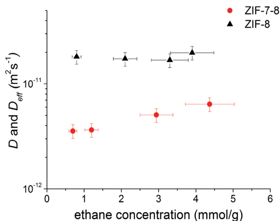
Fig. 2 Effective self-diffusion coefficients ( D_{\text{eff}} ) in ZIF-7-8 (red circles) and self-diffusion coefficients ( D ) in ZIF-8 (black triangles) for ethane measured by PFG NMR at 296 K as a function of the ethane concentration in the ZIF crystals.
