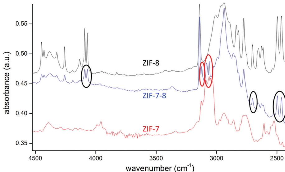
Fig. 3 Comparison of IR spectra of a ZIF-7, ZIF-8 and ZIF-7-8 crystal. In ZIF-7-8, the IR bands at 4100, 2700 and 2475 \text{cm}^{-1} are related to ZIF-8 (mIm), while the signals at 3115 and 3060 \text{cm}^{-1} are ascribed to ZIF-7 (bIm).
