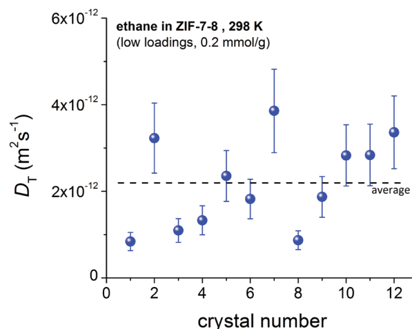
Fig. 4 Transport diffusivities, D_T , of ethane in ZIF-7-8 at 298 K measured for different individual crystals at low loadings. The diffusivities were found to scatter by a factor of up to 4.4.
