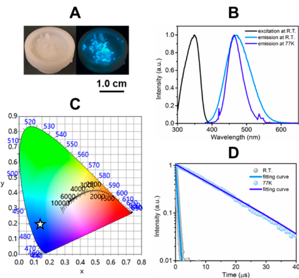
Figure 2. (A) Images of (\text{C}_9\text{NH}_{20})_7(\text{PbCl}_4)\text{Pb}_3\text{Cl}_{11}\cdot\text{CH}_3\text{CN} single crystals under ambient light and 365 nm UV irradiation. (B) Excitation and emission spectra of the single crystals at room temperature and 77 K. (C) CIE chromaticity coordinates (0.14, 0.19) of the blue emission from the single crystals plotted on the CIE 1931 color space chromaticity chart. (D) The emission decay curves at room temperature and 77 K.
