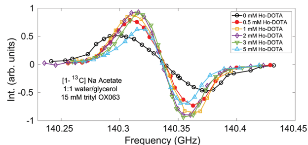
Fig. 1 ^{13}\text{C} DNP frequency sweeps of [ ^{13}\text{C} ] sodium acetate in 1:1 (v/v) water/glycerol solution in the presence of trityl OX063 radical for various concentrations of Ho-DOTA (0, 0.5, 1, 2, 3, 5 mM).
