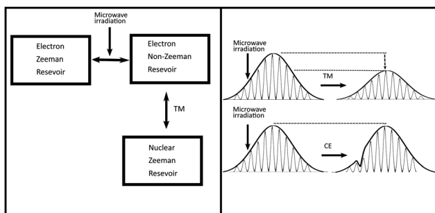
Fig. 3 Left panel: Schematic diagram of thermal mixing (TM), where a model of three interdependent spin baths is invoked. Right panel: The difference between the TM (complete saturation of the ESR line) and the cross effect (CE), where electron spectral diffusion is limited.
