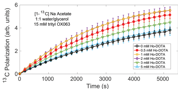
Fig. 2 ^{13}\text{C} polarization buildup curves of [1-^{13}\text{C}] sodium acetate in 1:1 (v/v) water/glycerol solution for different concentrations of Ho-DOTA (0, 0.5, 1, 2, 3, 5 mM) at the P(+) maximum peak position.
