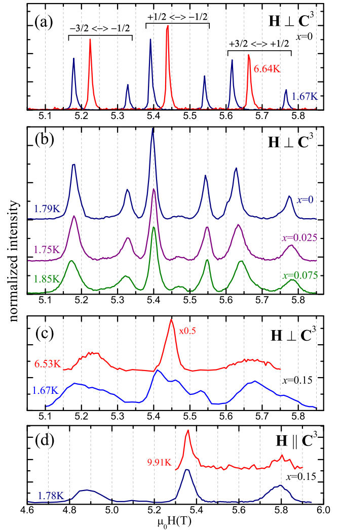
FIG. 2. ^{87}\text{Rb} NMR spectra of \text{Rb}_{1-x}\text{K}_x\text{Fe}(\text{MoO}_4)_2 , \nu = 75.5 \text{ MHz} , (a)–(c) \mathbf{H} \perp \mathbf{C}^3 , (d) \mathbf{H} \parallel \mathbf{C}^3 .
