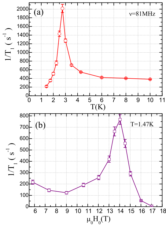
FIG. 5. (a) Temperature dependence of ^{87}\text{Rb} spin lattice relaxation rate T_1^{-1} in \text{Rb}_{0.85}\text{K}_{0.15}\text{Fe}(\text{MoO}_4)_2 at field 5.82 T, \mathbf{H} \perp \mathbf{C}^3 . (b) Field dependence of ^{87}\text{Rb} spin lattice relaxation rate T_1^{-1} in \text{Rb}_{0.85}\text{K}_{0.15}\text{Fe}(\text{MoO}_4)_2 at temperature 1.47 K, \mathbf{H} \perp \mathbf{C}^3 .
