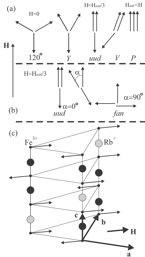
FIG. 1. (a) Magnetic structures expected for the XY TLAF with an in-plane external field as the field increases. (b) Magnetic structures with the total magnetization M = M_{sat}/3 . (c) Crystal structure of RbFe(MoO_4)_2 . The small circles are the positions of Fe^{3+} magnetic ions, the bigger circles (both black and gray, see text) are the positions of Rb^+ ions, the (MoO_4)^{2-} complexes are not shown. One magnetic cell of the uud phase is shown. \mathbf{a} , \mathbf{b} , and \mathbf{c} are the basis vectors describing the crystallographic structure; \mathbf{a} , \mathbf{b} are directed along the sides of the triangle while \mathbf{c} is aligned along C^3 . The translational vectors of the uud structure are \mathbf{a} + 2\mathbf{b} and 2\mathbf{a} + \mathbf{b} . The short arrows depict the expected orientations of magnetic moments in the uud phase with a period of 3c for the direction of the magnetic field \mathbf{H} as shown.
