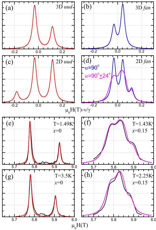
FIG. 6. Simulated NMR spectra corresponding to the uud structure ( \alpha = 0^\circ , left panels) and the fan structure ( \alpha = 90^\circ , right panels), \mathbf{H} \perp \mathbf{C}^3 . For comparison experimental ^{87}\text{Rb} NMR spectra (black lines) at frequency 81 MHz, \mathbf{H} \perp \mathbf{C}^3 , and two temperatures are shown for (e),(g) x = 0 and (h),(f) x = 0.15 . Simulated spectra data: (a) 3D uud with periodicity 2c or 3c in the \mathbf{C}^3 direction, \mu = 5\mu_B , individual linewidth \delta = 20 mT; (b) 3D fan with periodicity 2c or 3c in the \mathbf{C}^3 direction, \mu = 5\mu_B , \delta = 20 mT; (c) 2D uud , \mu = 5\mu_B , \delta = 20 mT; (d) 2D fan , \mu = 5\mu_B , \alpha = 90^\circ (blue line), \alpha = 90^\circ \pm 24^\circ (magenta line), \delta = 20 mT; (e) 3D uud , \mu = 5\mu_B , \delta = 6 mT; (f) 2D fan , \mu = 3.7\mu_B , \alpha = 90^\circ \pm 24^\circ , \delta = 20 mT; (g) 3D uud , \mu = 4.2\mu_B , \delta = 7 mT; (h) 2D fan , \mu = 3.3\mu_B , \alpha = 90^\circ \pm 22^\circ , \delta = 20 mT.
