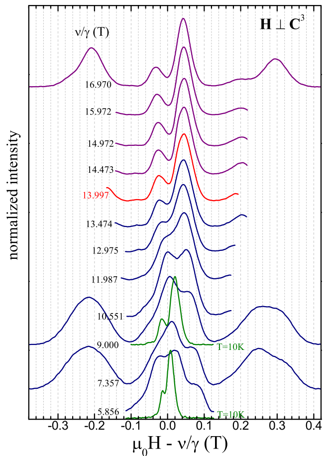
FIG. 4. Field evolution of ^{87}\text{Rb} NMR spectra in \text{Rb}_{0.85}\text{K}_{0.15}\text{Fe}(\text{MoO}_4)_2 at temperature \approx 1.47 K, \mathbf{H} \perp \mathbf{C}^3 . The spectrum shown with red line corresponds to the maximum of ^{87}\text{Rb} spin lattice relaxation rate T_1^{-1} shown in Fig. 5(b). The green colored spectra correspond to paramagnetic state ( T = 10 K).
