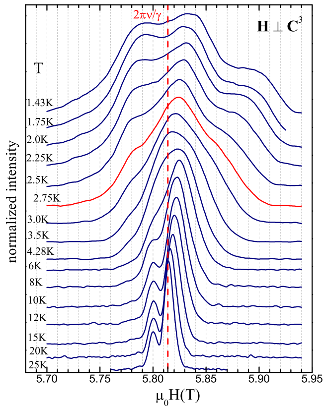
FIG. 3. Temperature evolution of ^{87}\text{Rb} NMR spectra ( m_I = +1/2 \leftrightarrow -1/2 transition) in \text{Rb}_{0.85}\text{K}_{0.15}\text{Fe}(\text{MoO}_4)_2 , \nu = 81 MHz, \mathbf{H} \perp \mathbf{C}^3 . The spectrum shown with red line corresponds to the maximum of ^{87}\text{Rb} spin lattice relaxation rate T_1^{-1} shown in Fig. 5(a).
