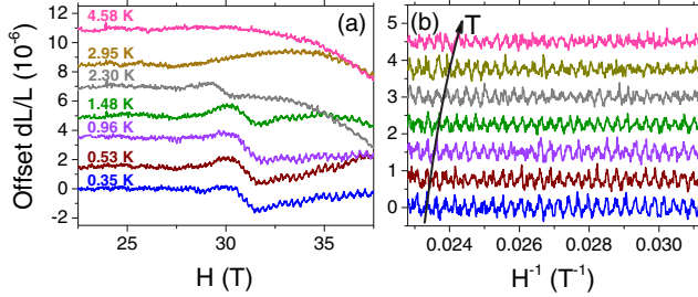
FIG. 4. (a) Temperature dependence of the magnetostriction of CeRhIn 5 for fields applied \approx 20^\circ off the c axis. An offset is added for clarity. (b) High-field quantum oscillations in inverse field obtained from the data shown in panel (a). The color scheme is the same in both panels.
