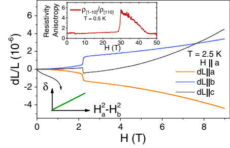
FIG. 1. Magnetostriction of CeRhIn 5 along the a axis, dL_a/L_a , at 2.5 K for fields applied in the tetragonal ab plane. Top inset shows the in-plane anisotropy in electrical resistivity [4]. Bottom inset shows a schematic diagram of the order parameter \delta as a function of the in-plane symmetry breaking field indicating that there is no intercept when the in-plane field goes to zero (see also Supplemental Material [20]).
