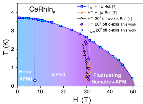
FIG. 5. H - T phase diagram of CeRhIn 5 . Data from Ref. [7] were obtained by specific heat and Hall measurements. Data from Ref. [4] were obtained by electrical resistivity.
