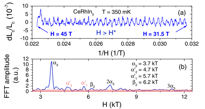
FIG. 3. (a) Magnetostriction of CeRhIn 5 at 350 mK as a function of inverse field for fields applied \approx 20^\circ off the c axis. A high-pass filter was used to remove low-frequency oscillations that likely originate from the background difference below and above H^* . (b) FFT spectra in the region 31.5 < H < 45 T. The dashed area is an estimate of the noise floor.
