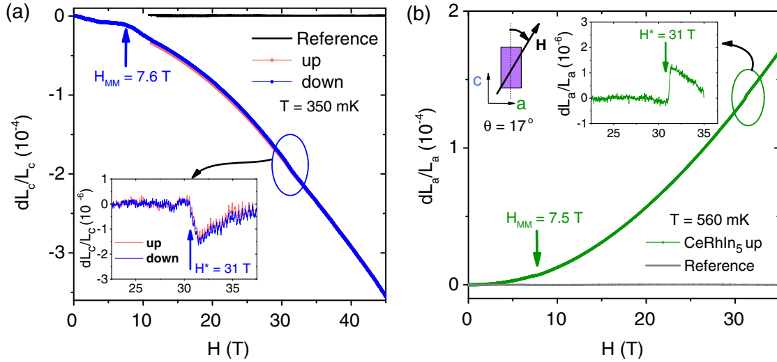
FIG. 2. Magnetostriction of CeRhIn 5 along (a) the c axis at T = 350 mK and (b) the a axis at T = 560 mK for fields applied \approx 20^\circ off the c axis. Here \theta is the polar angle between the applied field and the c axis. The azimuthal angle is set to \phi = 90^\circ . Insets show the data after a background subtraction.
