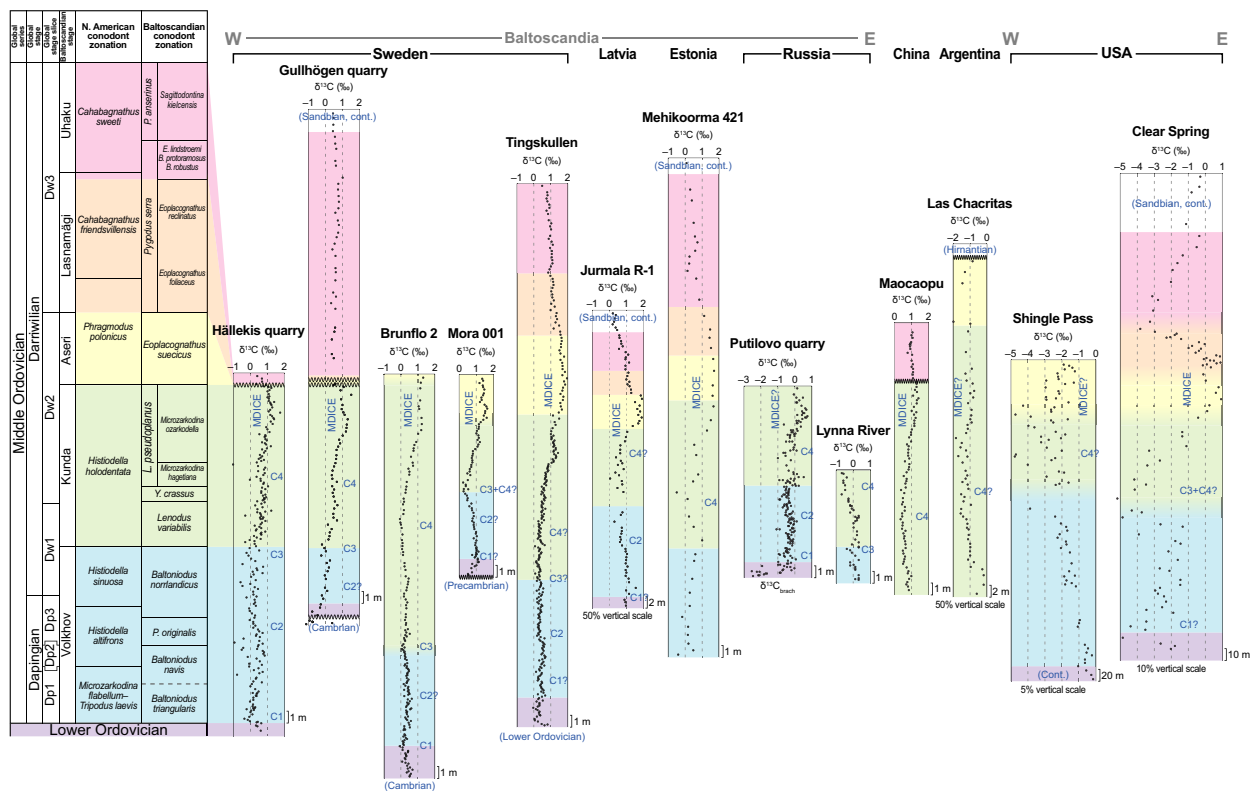
Fig. 5. Comparison between the carbon isotope ( \delta^{13}\text{C}_{\text{carb}} ) curve at Hällekis with (portions of) select \delta^{13}\text{C}_{\text{carb}} curves from other localities (Gullhögen quarry, outcrop: Meidla et al. 2004; Brunflo 2, drill core: Wu et al. 2017; Mora 001, drill core: Lehnert et al. 2014; Tingskulen, drill core: Wu et al. 2017; Jurmala R-1, drill core: Ainsaar et al. 2004; Mehikoorma 421, drill core: Kaljo et al. 2007; Putilovo quarry, outcrop: Rasmussen et al. 2016; Lynna River, outcrop: Zaitsev & Pokrovsky 2014; Maocaapu, outcrop: Schmitz et al. 2010; Las Chacritas, outcrop: Albanesi et al. 2013; Shingle Pass, outcrop: Edwards & Saltzman 2014; Clear Spring, outcrop: Saltzman & Edwards 2017). All sections are shown to the same vertical scale (i.e. their relative thicknesses are represented correctly), except where noted. Colour coding indicates biostratigraphical correlation as tied to the Baltoscandian stratigraphical framework (modified from Lindskog et al. 2017); graded transitions indicate uncertain boundaries (biostratigraphical data from Jaanusson & Mutvei 1951; Jaanusson 1964; Karis 1998; Zhang 1998a; Löfgren 2003; Ainsaar et al. 2004; Meidla et al. 2004; Bergström 2007; Kaljo et al. 2007; Schmitz et al. 2010; Albanesi et al. 2013; Edwards & Saltzman 2014; Rasmussen et al. 2016; Lindskog & Eriksson 2017; Saltzman & Edwards 2017; Wu et al. 2017; see further references therein). [Colour figure can be viewed at wileyonlinelibrary.com ]
