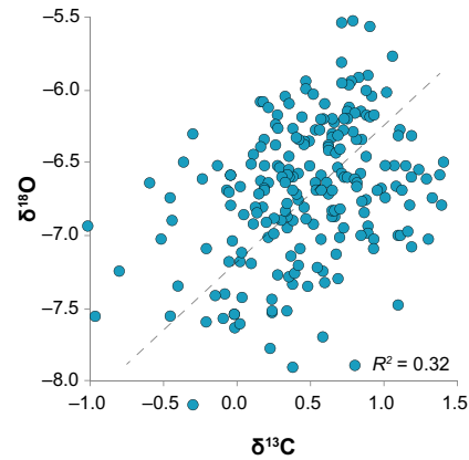
Fig. 4. Cross-plot of the \delta^{13}\text{C} and \delta^{18}\text{O} data with linear (least-squares regression) trend line indicated. [Colour figure can be viewed at wileyonlinelibrary.com ]
