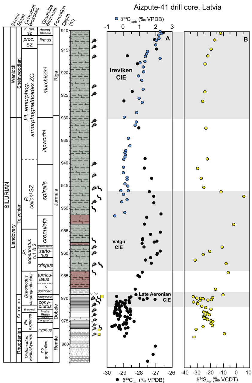
Fig. 4. Llandovery–early Wenlock (early Silurian) stable isotopic data ( \delta^{13}C_{org} and \delta^{34}S_{pyr} ) from the Aizpute-41 drill core, Latvia. Graptolite and conodont biozones are plotted from previous biostratigraphic studies (Loydell et al., 2003; Cramer et al., 2010). The \delta^{13}C_{carb} data (blue circles) are replotted from Cramer et al. (2010). Please refer to legend in Fig. 2 for lithology and fossil symbols used. Grey bars denote globally documented positive carbon isotope excursions (CIEs). (For interpretation of the references to colour in this figure legend, the reader is referred to the web version of this article.)
