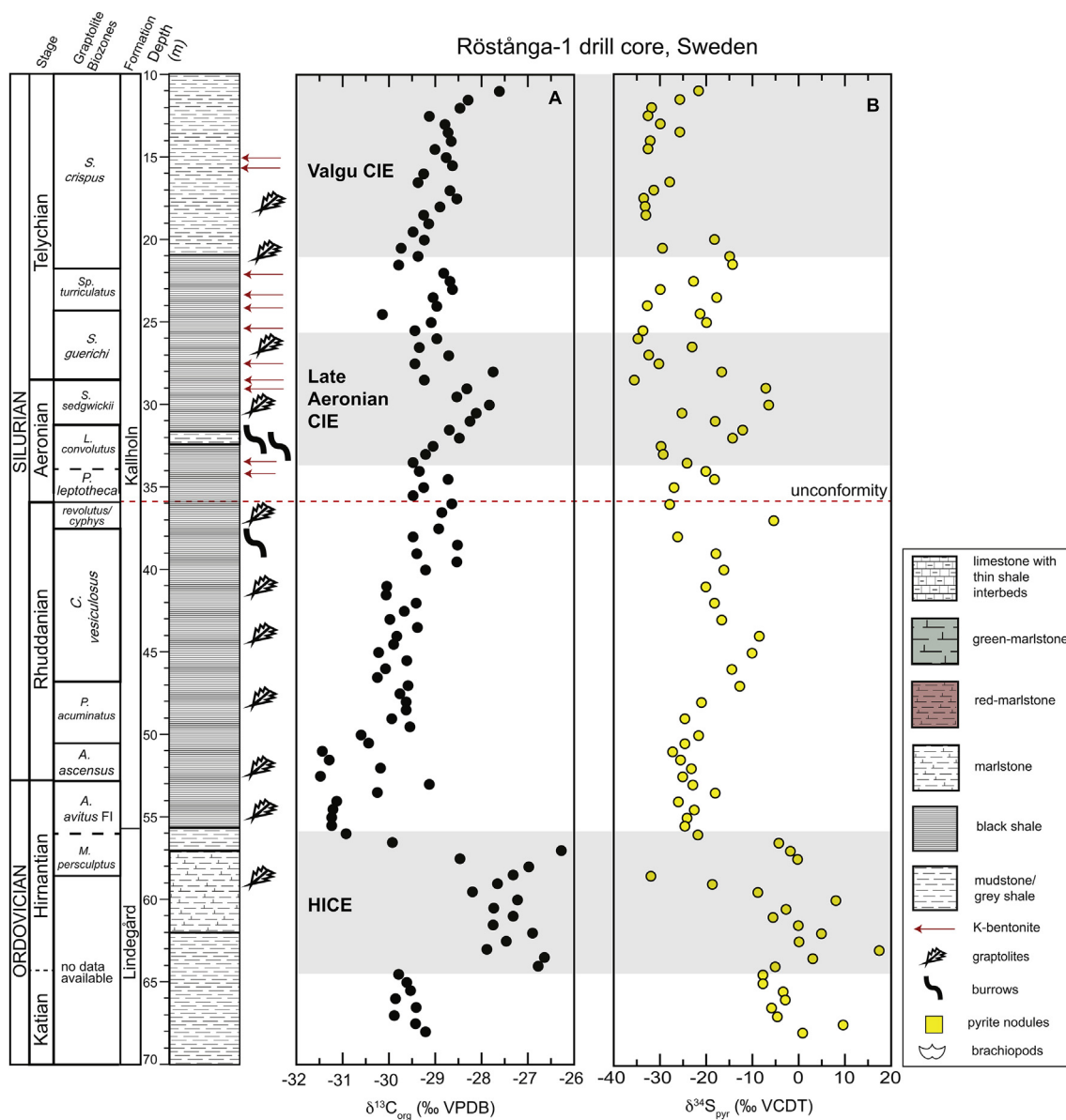
Fig. 2. Late Ordovician–early Silurian stable isotopic data ( \delta^{13}\text{C}_{\text{org}} and \delta^{34}\text{S}_{\text{pyr}} ) from the Röstånga-1 drill core, Sweden. Graptolite biozones are plotted from previous biostratigraphic studies (Bergström et al., 1999; Koren et al., 2003; Maletz et al., 2014). Grey bars denote globally documented positive carbon isotope excursions (CIEs), including the HICE–Hirnantian carbon isotope excursion.
