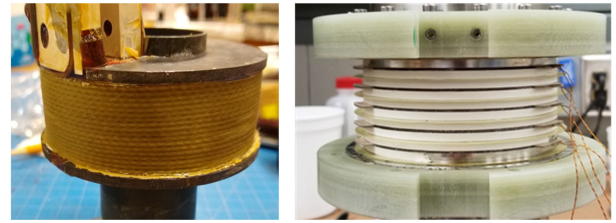
Fig. 6. A Bi-2212 test coil (left) and an NI-REBCO test coil (right). The Bi-2212 coil was tested in a 14 T LTS magnet. The NI-REBCO with 6 DPs was tested in a 6.9 T background field.
