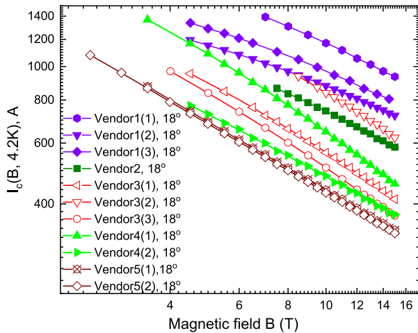
Fig. 2. Characterization of REBCO tapes (4 mm width) from various vendors. The I_c was measured at various magnetic fields, field angles and temperatures. This plot shows the I_c up to 15 T at 4.2 K and an angle of 18 degree from the tape plane. The tape characterization is necessary to identify potential vendors for high field magnets conductors and to provide I_c data for 40 T SC magnet designs. The I_c variation of vendor 3 is due to intentional grading.
