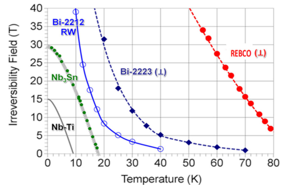
Fig. 1. Irreversibility field of the superconducting conductors. Each of the three HTS conductors (Bi-2212, Bi-2223 and REBCO) has an irreversibility field well above the limit that LTS conductors (Nb-Ti and Nb 3 Sn) can reach [4].
