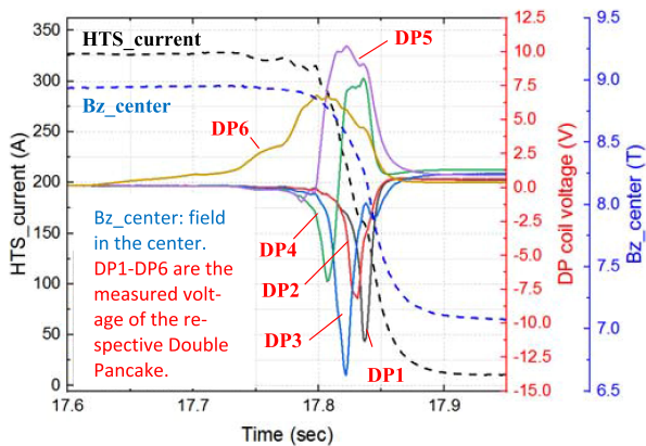
Fig. 5. Quench transient process of an NI test coil. This coil was tested in a background field of 6.9 T to investigate the fatigue life of a REBCO coil. The quench initiated in Double-Pancake 6 (DP6).
