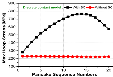
Fig. 4. Simulated maximum hoop stress in a pancake REBCO coil: with and without consideration of screening current (SC). They are calculated using COMSOL with discrete contact elements [32].
