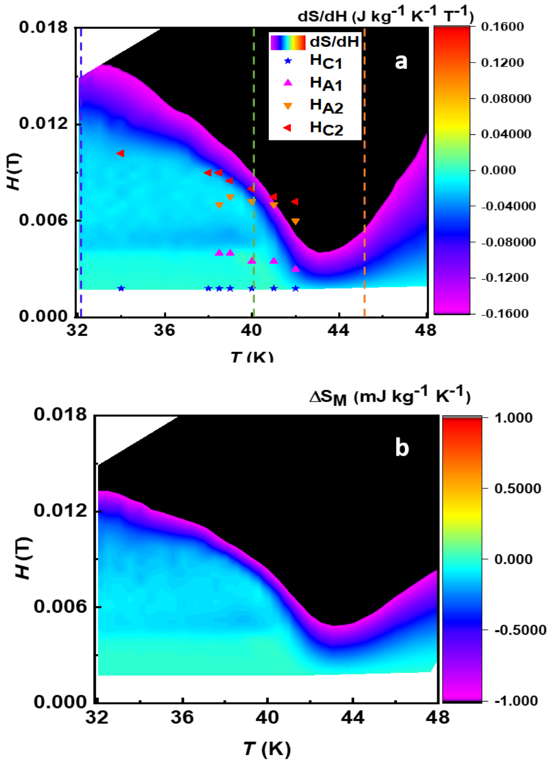
Fig. 7 Color maps of \text{Fe}_{0.7}\text{Co}_{0.3}\text{Si} (a) dS/dH as function of T and H (b) \Delta S_M as function of T and H . Here H refers to the internal field after correcting for demagnetization fields as described in supplemental section [28].
