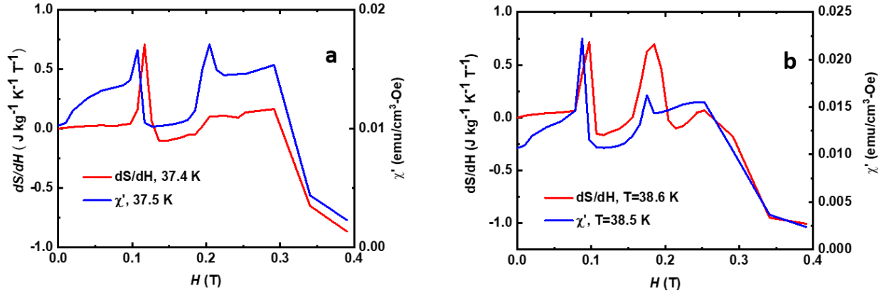
Fig. S1. Comparison of real part of ac susceptibility, \chi' and dS/dH for \text{MnSi}_{0.962}\text{Al}_{0.038} (a) at T \sim 37.5 K (b) at T \sim 38.5 K.
