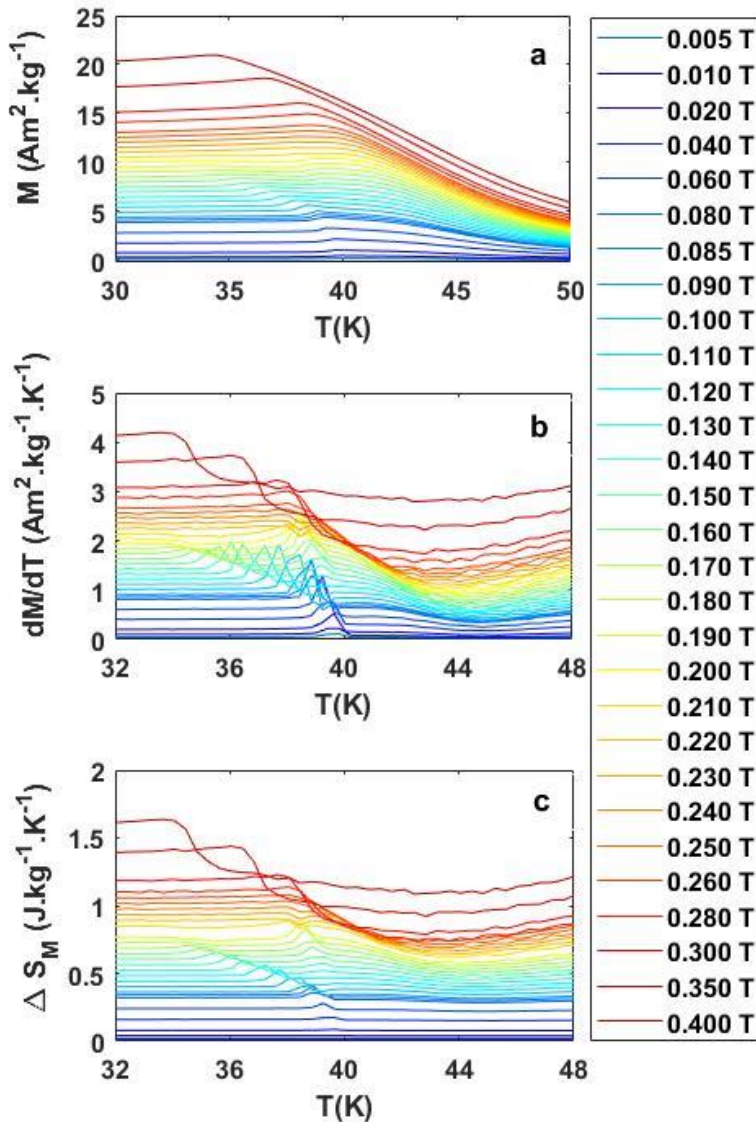
Fig. 2 Magnetic entropy changes in \text{MnSi}_{0.962}\text{Al}_{0.038} . (a) Magnetization, M , as function of temperature, T for a range of applied magnetic field between H_a= 0.005 and H_a = 0.4 T. (b) The
