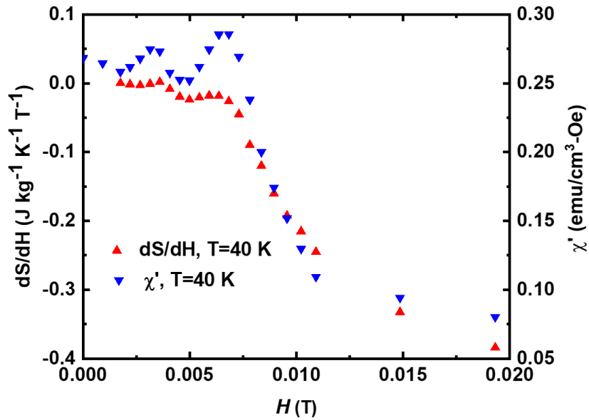
Fig. S2. Comparison of real part of ac susceptibility, \chi' and dS/dH for \text{Fe}_{0.7}\text{Co}_{0.3}\text{Si} .
