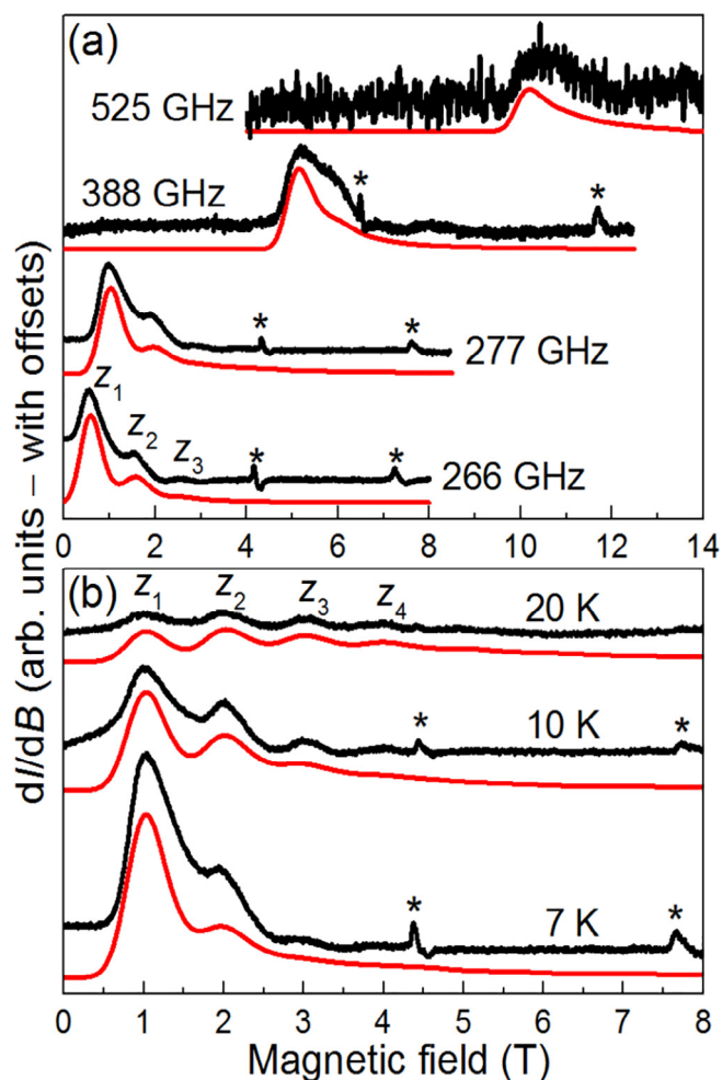
Fig. 14. (a) Frequency-dependent HFEPR spectra (black) for a vacuum-dried polycrystalline powder sample of 5 \cdot 3/2 hexane at T = 7 K. (b) Temperature dependence of the 277.1 GHz spectrum in (a). Simulations (red) are shown below each experimental trace in both (a) and (b); see text for obtained zfs parameters. Up to four resonances can be identified that are associated with the parallel ( H//z ) component of the full spectrum; these are labeled z_1 to z_4 , corresponding to the m_S = -19/2 \rightarrow -17/2, -17/2 \rightarrow -15/2, -15/2 \rightarrow -13/2, and -13/2 \rightarrow -11/2 transitions (see Fig. S8). Features marked with an asterisk are due to a known frozen molecular oxygen contaminant in the sample holder.
