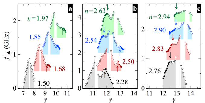
FIG. 10. (a)–(c) f_{pk} vs. \gamma at various n , as marked, for \theta = 0^\circ . Traces are vertically offset from one another for clarity and shaded to f_{pk} = 0 . \uparrow and \downarrow mark the S2-S1 transition for \nu < 1 and \nu > 1 , respectively.
