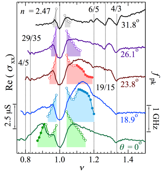
FIG. 9. Real part of the conductivity, \text{Re}(\sigma_{xx}) , obtained at fixed frequency, f = 0.5 GHz, vs. \nu (left axis) at various \theta as marked. For each \theta , f_{pk} vs. \nu (right axis) shaded to f_{pk} = 0 . Traces are vertically offset for clarity. The vertical lines mark \nu = 4/5, 1, 6/5 , and 4/3 , as well as 29/35 and 19/15 .
