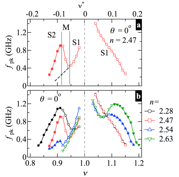
FIG. 3. Data for Sample B. (a) f_{\text{pk}} vs. \nu for n = 2.47 , tilt angle \theta = 0^\circ . The regions of solids S1, S2 are marked, as is the region (M) of transition between S1 and S2. Symbols within well-developed S2 are filled. (b) f_{\text{pk}} vs. \nu at different n with sample perpendicular to magnetic field, \theta = 0^\circ . For \nu > 1 the data for n = 2.28 lie directly under those for n = 2.47 .
