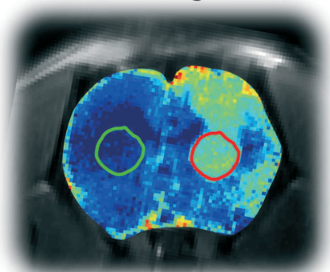
CEST-weighted
