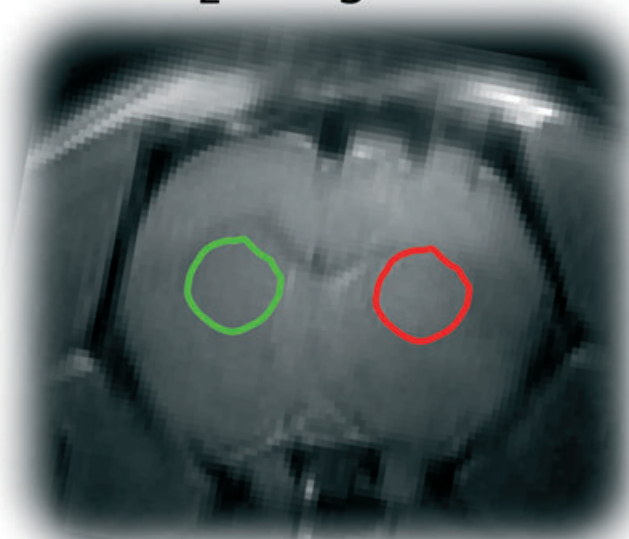
T 2 -weighted
