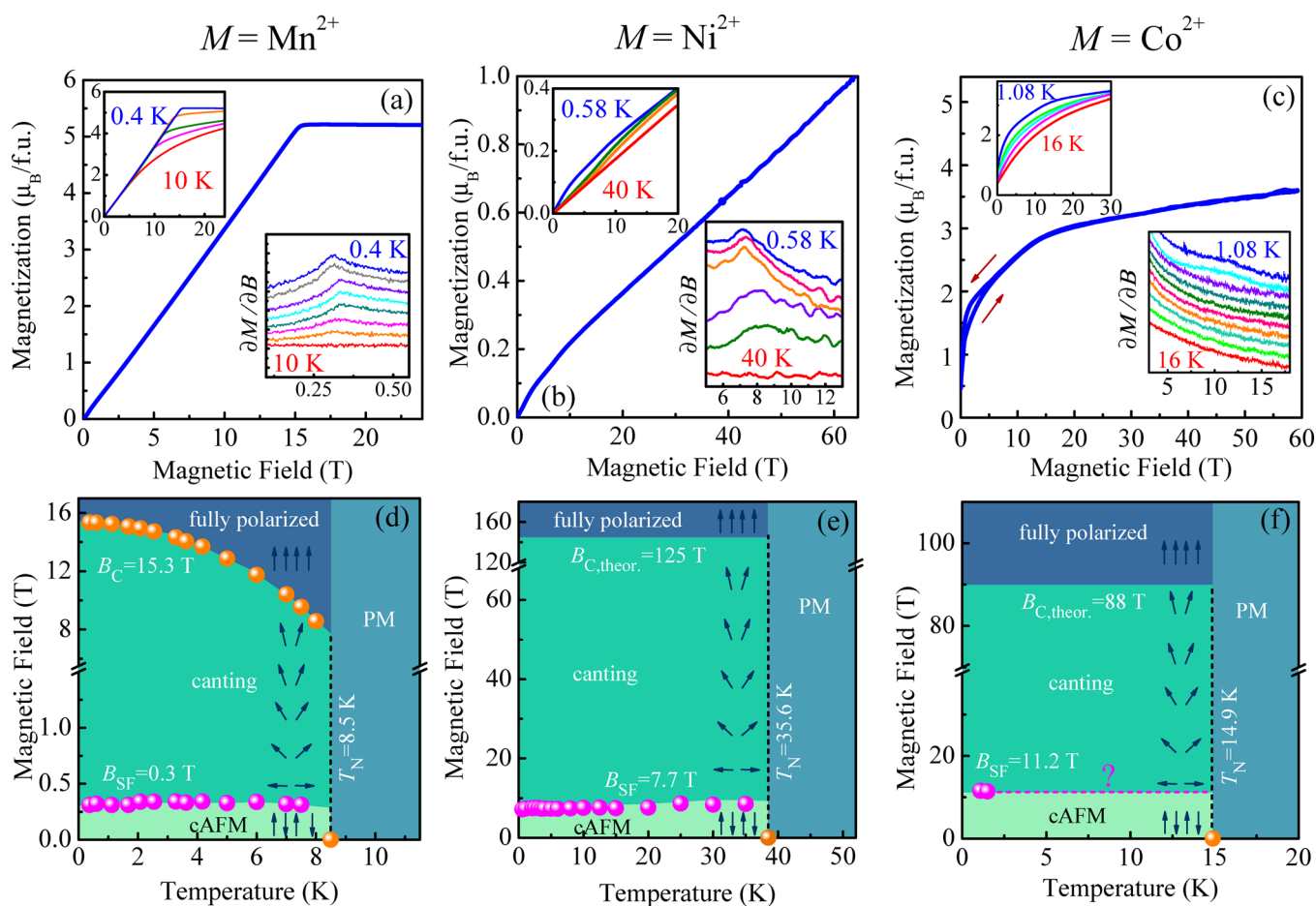
Figure 2. (a–c) Pulsed field magnetization of [(\text{CH}_3)_2\text{NH}_2]\text{M}(\text{HCOO})_3 ( M = \text{Mn}^{2+} , \text{Co}^{2+} , \text{Ni}^{2+} ) up to 65 T at different temperatures. Derivatives of this data reveal B_{\text{SF}} as shown in the lower insets. Only the Mn compound has a clear saturation field under these conditions. 13 The Ni and Co systems are not saturated even at 65 T. (d–f) Magnetic field-temperature phase diagrams developed from the pulsed field magnetization data. Orange points denote the transition to the fully saturated magnetic state, and pink points indicate the spin flop. The high field phase boundaries for the Ni and Co compounds are estimated as described in the text. Error bars are on the order of the symbol size. cAFM = canted antiferromagnet, and PM = high-temperature paramagnetic state.
