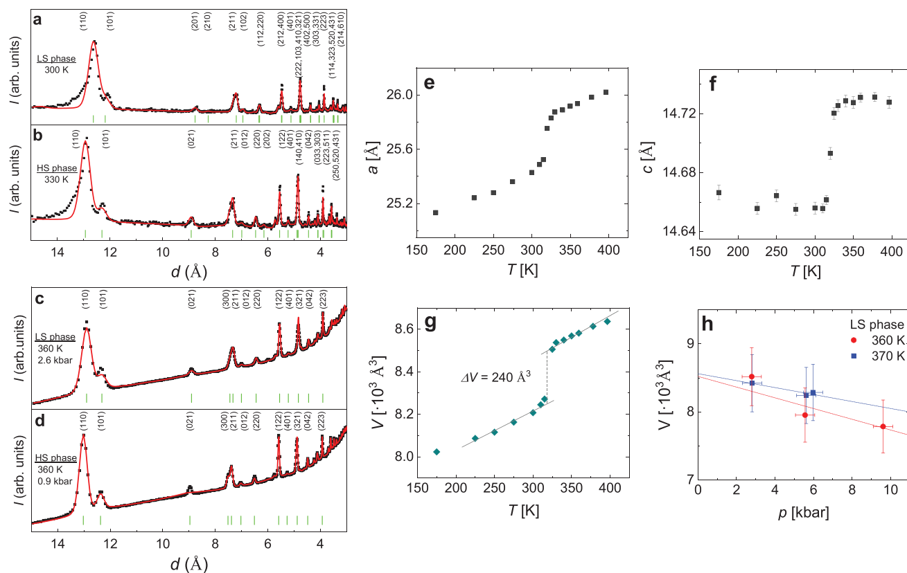
Figure 2. a,b) Ambient-pressure powder diffraction patterns at T = 300 K (a) and T = 330 K (b). c,d) Isothermal ( T = 360 K) powder diffraction patterns at p = 2.6 kbar (c) and p = 0.9 kbar (d). (a,c) and (b,d) correspond to the LS and HS states, respectively. The solid symbols correspond to experimental data, the red lines correspond to the theoretical powder diffraction pattern profiles calculated by the Pawley method, and the green lines indicate the position of the Bragg peaks, whose (hkl) Miller indices are indicated at the top of each panel. e–g) Ambient pressure temperature evolution of the lattice parameters (e,f) and the unit cell volume (g). h) Pressure dependence of the unit cell volume at selected values of temperature. Lines are linear fits to the data.
