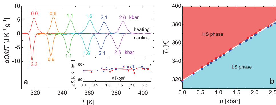
Figure 4. a) Temperature-dependent isobaric heat flow dQ/dT at different pressures, after baseline subtraction. The upper and lower curves correspond, respectively, to the endothermic LS to HS transition on heating and to the exothermic HS to LS transition on cooling. The inset shows the transition entropy change as a function of pressure. Blue symbols correspond to the HS to LS transition and red symbols, to the LS to HS transition. b) Transition temperature (peak in the calorimetric curves) as a function of hydrostatic pressure. The blue symbols correspond to the HS to LS transition and the red symbols, to the LS to HS transition. The lines are linear fits to the data.
