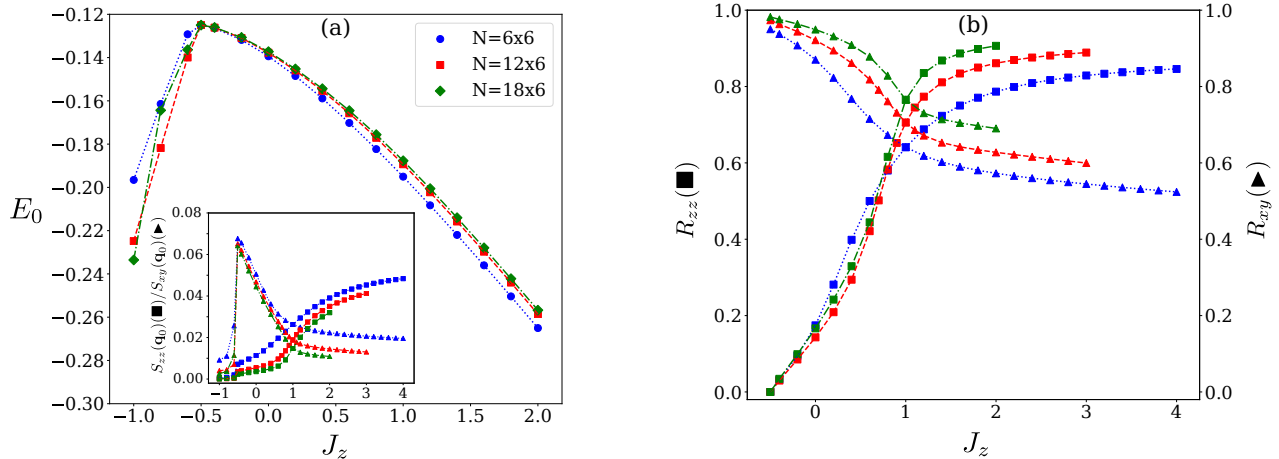
Figure 4. For the triangular lattice XXZ Hamiltonian in the m = 0 sector, the left panel shows the ground state energy per bond ( E_0 ) vs. J_z . The inset of the left panel shows the evolution of the structure factors ( \frac{S_{zz}(\mathbf{q}_0)}{N} and \frac{S_{xy}(\mathbf{q}_0)}{N} ), calculated at the ordering vector \mathbf{q}_0 = (4\pi/3, 0) . The right panel shows the correlation ratios ( R_{zz} and R_{xy} ), as defined in the text (Eq. 10), vs. J_z at the ordering wave-vector \mathbf{q}_0 for the representative case of \Delta\mathbf{q} = (\frac{2\pi}{L_x}, \frac{4\pi}{\sqrt{3}L_y} - \frac{2\pi}{\sqrt{3}L_x}) .
