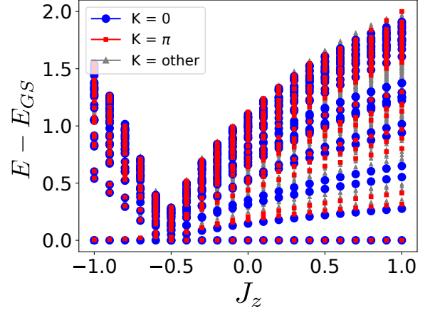
Figure 9. Energy spectrum of the 18 site periodic anisotropic Majumdar-Ghosh chain as a function of J_z ( J_1 = 1 ) in the S_z = 0 sector. For a given J_z , only the lowest 30 energies in each momentum sector are plotted. The ground state energy is subtracted out at each value of J_z . There is a phase transition at J_z = -\frac{1}{2} . For J_z > -\frac{1}{2} the ground state is exactly two fold degenerate (one state in k = 0 and the other in k = \pi ), which correspond to linear combinations of the two Majumdar-Ghosh dimer (valence bond) solutions. These ground states persist all the way to the Heisenberg point ( J_z = 1 ) and beyond (not shown), consistent with the analytic arguments.
