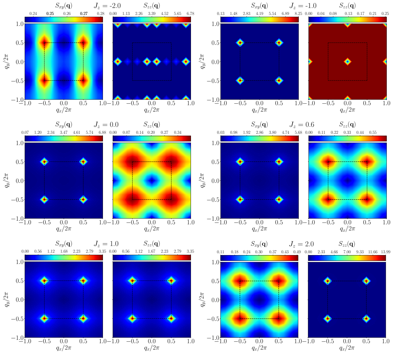
Figure 3. The panels show S_{xy}(\mathbf{q}) and S_{zz}(\mathbf{q}) for the square lattice, in the first Brillouin zone (highlighted by the dashed black lines) for various representative J_z in the m = 0 magnetization sector for the N = 8 \times 8 cylinder.
