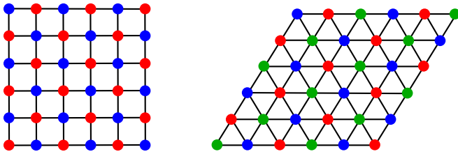
Figure 1. Illustration of the unique two-coloring on the square lattice, and one of the two three-colorings on the triangular lattice. The colorings directly correspond to magnetically ordered states.
