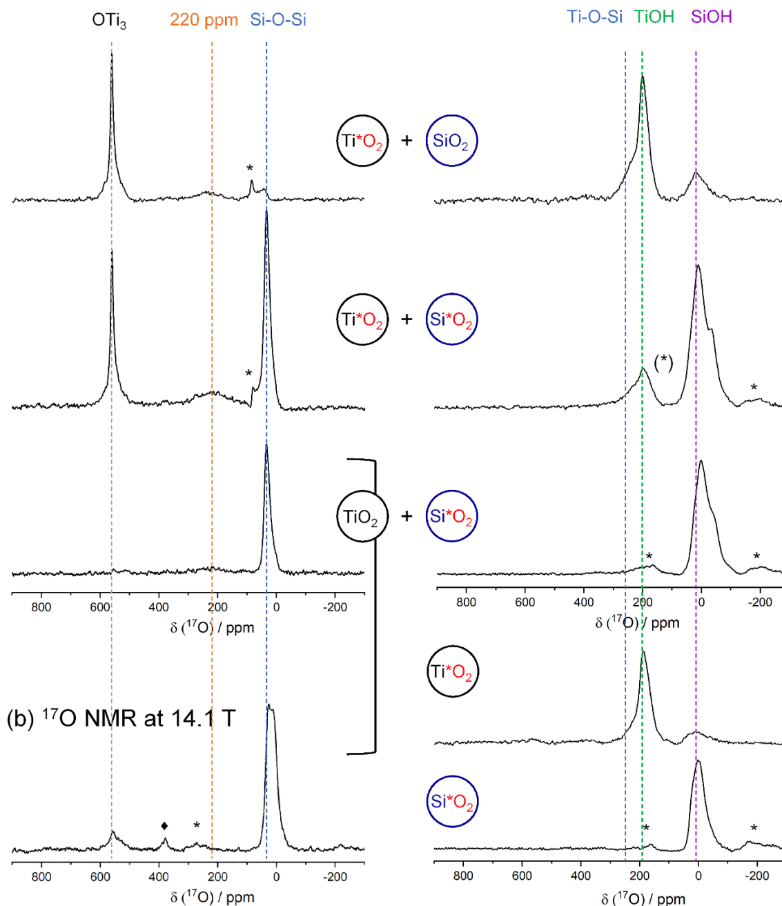
Figure 6. (a) ^{17}\text{O} polarization-enhanced spin-echo NMR spectra of \text{Ti}^*\text{O}_2 + \text{SiO}_2 [33] , \text{Ti}^*\text{O}_2 + \text{Si}^*\text{O}_2 , and \text{TiO}_2 + \text{Si}^*\text{O}_2 (20.0 T, 55 kHz MAS). The temperature of ^{17}\text{O} NMR spectra of \text{Ti}^*\text{O}_2 + \text{Si}^*\text{O}_2 , and \text{TiO}_2 + \text{Si}^*\text{O}_2 mixtures was controlled at 0°C. (b) ^{17}\text{O} DFS NMR spectrum of \text{TiO}_2 + \text{Si}^*\text{O}_2 (14.1 T, 20 kHz MAS) (c) ^{17}\text{O}\{^1\text{H}\} DNP CPMAS NMR of \text{Ti}^*\text{O}_2 + \text{SiO}_2 , \text{Ti}^*\text{O}_2 + \text{Si}^*\text{O}_2 , and \text{TiO}_2 + \text{Si}^*\text{O}_2 , \text{Ti}^*\text{O}_2 [33] , and \text{Si}^*\text{O}_2 . The contact time was 50 \mu\text{s} . (14.1 T, 13 kHz MAS). * indicates spinning sidebands and ♦ indicates zirconia rotor.
