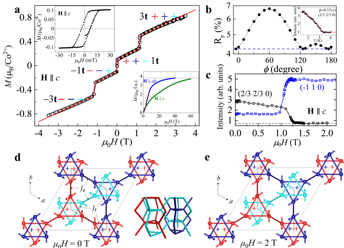
Fig. 2 Zero-field magnetic structure and field-induced ferri- to ferrotoroidal transition in \text{BaCoSiO}_4 . a The isothermal bulk magnetization data (open circles) measured at 2 K with the field parallel to the c -axis and the theoretical calculations (red line) from the full spin Hamiltonian, showing a good agreement between data and calculations. The magnetization up to 60 T in a pulsed magnetic field at 1.5 K is shown in the lower inset, and the magnetization hysteresis at low fields in the upper inset. See caption of panel (d) for the meaning of symbols + and -. b The refined agreement factor for the powder neutron diffraction data as a function of uniform rotation in the ab plane. The dashed line marks the best refinement. Inset shows the integrated intensity of the magnetic reflection (2/3\ 2/3\ 0) as a function of temperature with an order parameter fit \sim (1 - T/T_N)^{2\beta} (solid line), where \beta is the critical exponent. The error bars are used to show the standard deviation given by the square root of the number of neutron counts. c The integrated intensities of reflection (2/3\ 2/3\ 0) and (-1\ 1\ 0) as a function of the magnetic field with \mathbf{H} \parallel c at 1.5 K. d Zero-field magnetic structure of \text{BaCoSiO}_4 in a \sqrt{3} \times \sqrt{3} supercell solved from powder neutron diffraction data, showing three interpenetrating ferrotoroidal sublattices (red, blue, and cyan) formed by the dominant exchange interactions J_i (intra-layer) and J_z (inter-layer). The direction of the toroidal moment for each sublattice is denoted + if it is parallel to the c -axis and - if antiparallel. The red and blue sublattices have the same toroidal moment, while the cyan has the opposite moment, leading to a ferritoroidal state with a total moment +1t . The primitive crystallographic unit cell is indicated by the dotted lines. e Magnetic structure of \text{BaCoSiO}_4 at 2 T solved from single-crystal neutron diffraction data. All spins on the cyan sublattice are reversed, leading to a ferrotoroidal state with a total toroidal moment +3t . Triangles in panels (d, e) lie in two adjacent layers, which are bridged by the interlayer interaction J_z .
