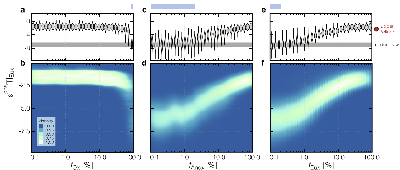
Fig. 5. Violin plots and two-dimensional heat maps illustrating the frequency distribution of modeled Tl isotope compositions of euxinic sediments ( \epsilon^{205}\text{Tl}_{Eux} ) as a function of logarithmically scaled oxic ( f_{Ox} ; a and b), anoxic ( f_{Anox} ; c and d), and euxinic ( f_{Eux} ; e and f) seafloor areal fraction in our statistical isotope mass balance model. The f_{Anox} is calculated as the sum of euxinic ( f_{Eux} ) and reducing ( f_{Red} ) seafloor areal fraction. The \epsilon^{205}\text{Tl}_{Eux} is calculated via the Monte Carlo analysis of marine Tl isotope mass balance. The \epsilon^{205}\text{Tl}_{Eux} of the upper Velkerri interval is labeled at the right-side panel with the red circle denoting the median value and error bars representing the data range. The dark grey bars across the violin plots denote the \epsilon^{205}\text{Tl} of the modern seawater. The blue shaded rectangles on top of violin plots represent the areal fractions of modern oxic, anoxic, and euxinic seafloor ( f_{Ox} : 84–94%; f_{Anox} : 0.1–2.0%; f_{Eux} : 0.1–0.2%), respectively.
