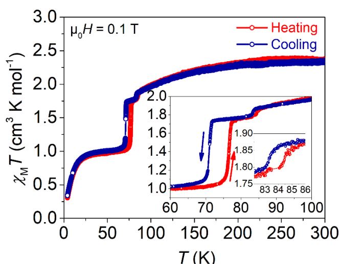
Figure 1. \chi_M T vs T measured at 0.1 T in a vibrating sample magnetometer (VSM) at 1 K/min on warming and cooling in a polycrystalline sample. A SCO occurs centered at 74 K with a hysteresis window of 6 K (larger inset). A second transition is observed at 84 K with a hysteresis window of ca. 1 K (smaller inset). \chi_M T saturates at 2.35 \text{ cm}^3 \cdot \text{K} \cdot \text{mol}^{-1} at room temperatures.
