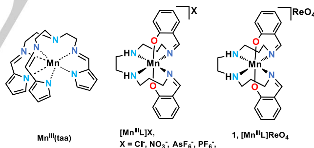
Scheme 1. Left: Structure of the most well-studied neutral Mn^{3+} SCO complex Mn(taa) . Middle: Structure of a Mn^{3+} complex cation, [Mn^{III}sal_2(323)]^+ , with an N_4O_2^{2-} ligand donor set which has previously shown to promote SCO with different charge balancing anions: Cl^- , NO_3^- , AsF_6^- , PF_6^- . [34,35] Right: Structure of [Mn^{III}sal_2(323)]ReO_4 , complex 1 .
