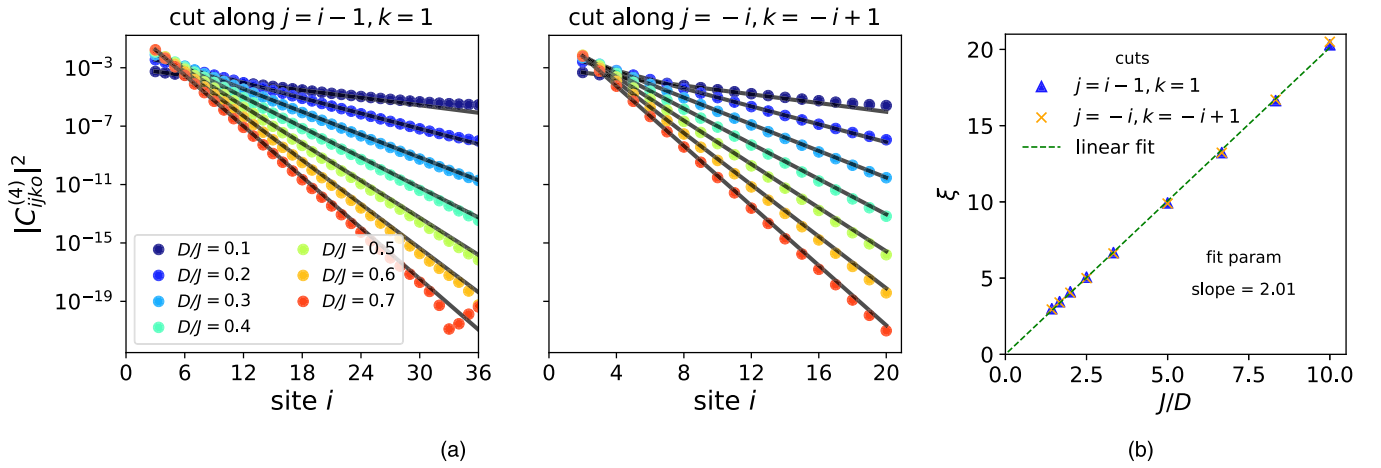
FIG. 9. The four-magnon correlator C_{ijk}^{(4)} , obtained by fixing one magnon at a reference site o , computed for the ground state of four magnons for representative values of anisotropy parameter D , in a periodic chain of length L = 76 . (a) The spatial dependence of the correlator for two one-dimensional cross sections, respectively corresponding to the two magnons at sites i and j with j = i - 1 and k = 1 (left panel), and j = -i and k = -i + 1 (right panel). Both cross sections show exponential decay with increasing spatial dependence between the magnons. Black solid lines are the fits with Jastrow factor \prod_{a<b} e^{lx_a - x_b/\xi} . (b) Correlation length \xi vs inverse anisotropy 1/D (with J = 1 ), obtained from fitting to the Jastrow form. Just as in the case of three magnons, here too the green dashed line shows that the linear fit is an excellent approximation to the four magnon correlator data.
