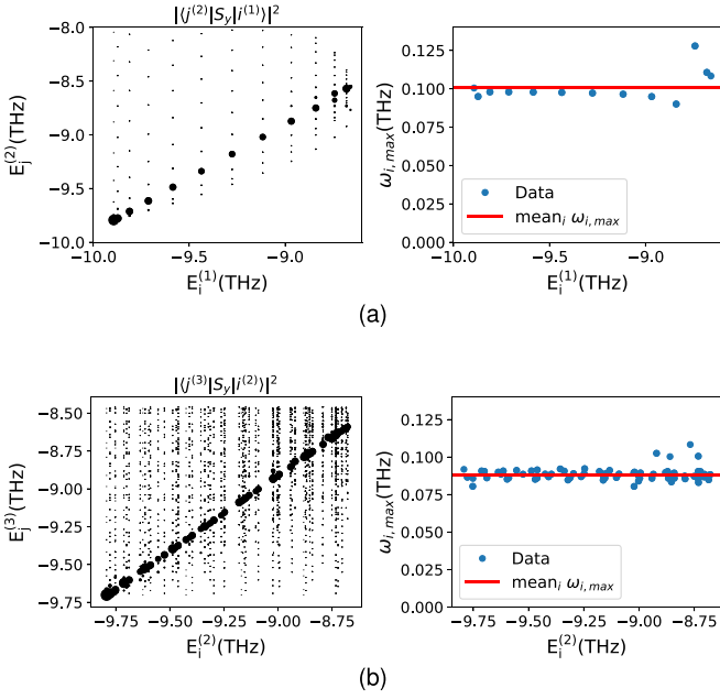
FIG. 6. Matrix elements |\langle j^{(n+1)}|S_y|i^{(n)}\rangle|^2 for transitions between (a) (left panel) for n = 1 and (b) (left panel) n = 2 magnon levels calculated in a periodic chain of length L = 24 using ED and for parameters relevant to \text{NiNb}_2\text{O}_6 , i.e., J = 0.308 THz and D = 0.108 THz. The size of each black dot represents the square of the absolute value of the corresponding matrix element. Right panels of both (a) and (b) represent the frequency \omega_{i,\max} at which the transitions in the left panels are most active for a given |i^{(n)}\rangle , i.e., corresponding to the |j^{(n+1)}\rangle with the largest absolute value of the matrix element |\langle j^{(n+1)}|S_y|i^{(n)}\rangle|^2 .
