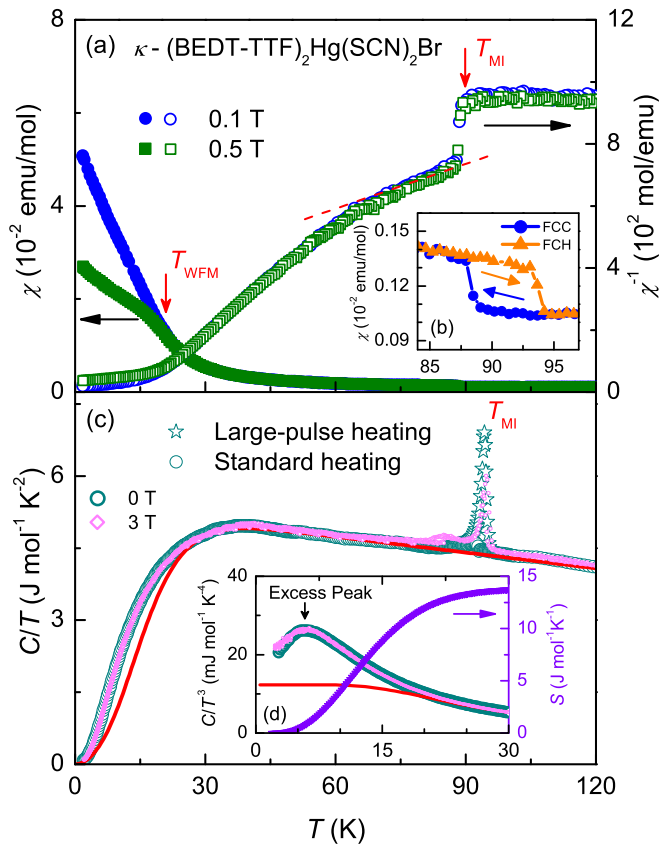
FIG. 5. (a) Temperature dependence of the magnetic susceptibility of an assembly of crystals (left ordinate) and its inverse (right ordinate) measured at two different magnetic fields. (b) Hysteresis of the temperature-dependent susceptibility on cooling and heating through the MIT. (c) Temperature dependence of specific heat in a representation of C/T . The red solid line corresponds to the Debye-Einstein fit (see text). (d) C/T^3 vs T plot reveals an excess-heat capacity or excess peak. Both MIT and excess peak are robust at 3 T. The entropy S is obtained as 13.7 J/mol K.
