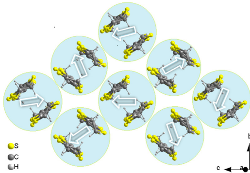
FIG. 1. Top view on the conductive bc planes of the dimerized BEDT-TTF molecules of \kappa -(BEDT-TTF) _2 Hg(SCN) _2 Br; each dimer hosts one spin. The dimer pattern can be modeled by an almost isosceles triangular lattice that is characterized by frustration effects. An artistic view of the spin arrangement illustrates that below the metal-insulator transition at T_{\text{MI}} \approx 90 K, spin frustration becomes dominant and suppresses the magnetic order.
