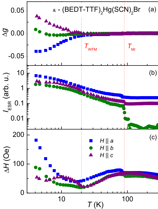
FIG. 3. Temperature dependence of ESR parameters (FC) of \kappa -(BEDT-TTF) _2 Hg(SCN) _2 Br for the magnetic field applied along the crystallographic principal axes: (a) g -shift \Delta g = g - g(300 \text{ K}) , (b) double integrated intensity I_{\text{ESR}} , and (c) linewidth \Delta H determined at X -band frequency. Red dotted lines indicate T_{\text{MI}} at 90 K and a weak ferromagnetic transition at T_{\text{WFM}} \approx 20 \text{ K} .
