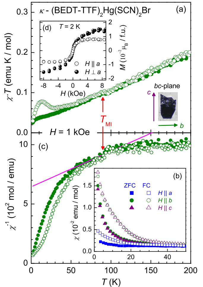
FIG. 4. (a) Temperature dependence of the susceptibility \chi of \kappa -(BEDT-TTF) _2 Hg(SCN) _2 Br in representation \chi \cdot T . (b) \chi(T) for the magnetic field H = 1 \text{ kOe} applied along the three principal crystallographic axes under zero-field-cooled (ZFC, solid symbols) and field-cooled (FC, open symbols) conditions. The inset depicts the single crystal under investigation. Note that the bc plane is the conductive plane. (c) Inverse susceptibility as a function of temperature. Straight lines indicate Curie-Weiss laws as discussed in the text. The inset (d) shows the field dependence of the magnetization at T = 2 \text{ K} .
