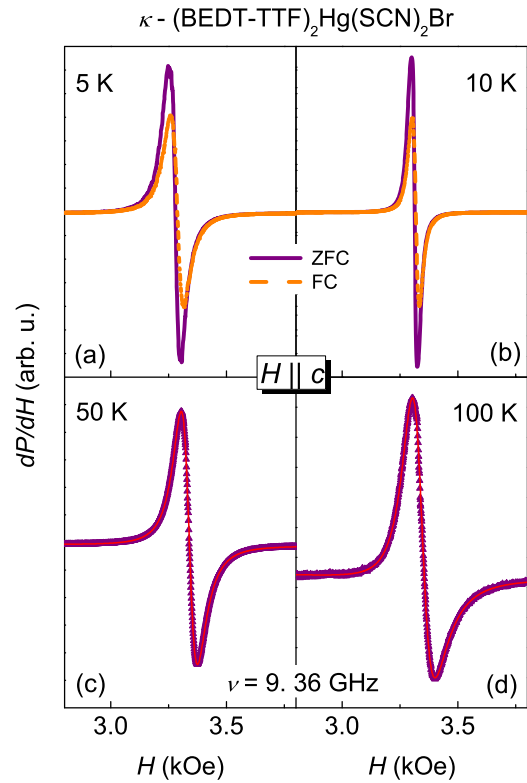
FIG. 2. ESR spectra, i.e., field derivative of absorbed power, of \kappa -(BEDT-TTF) _2 Hg(SCN) _2 Br taken at X-band frequency for selected temperatures and H \parallel c as indicated. Zero-field-cooled (ZFC) and field-cooled (FC) measurements (orange) are depicted in (a) and (b). The red solid lines, shown in (c) and (d), correspond to a fit by the field derivative of a Lorentz and Dyson line, respectively.
