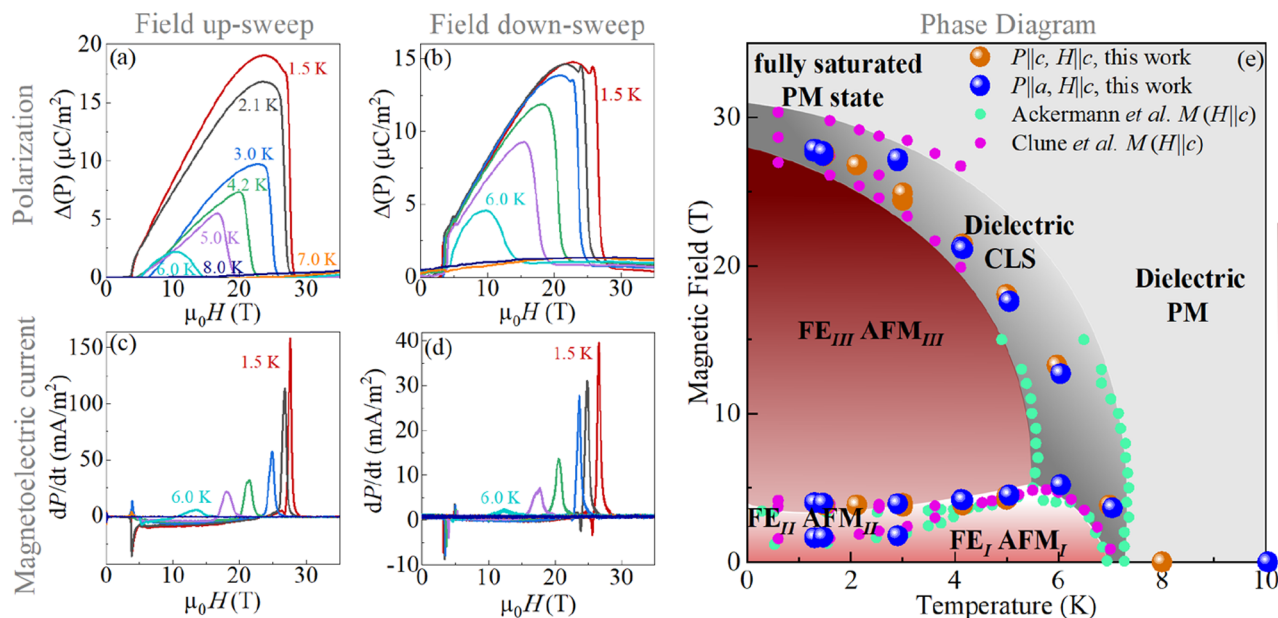
Figure 2. (a,b) Change in electric polarization ( \Delta P ) of (\text{NH}_4)_2[\text{FeCl}_5(\text{H}_2\text{O})] as a function of magnetic field (up- and down-sweeps) at various temperatures. This is the P\parallel c, H\parallel c configuration. Others are given in the Supporting Information. In each case, polarization is measured after poling the sample in an electric field. (c,d) Magneto-electric current I = dP/dt vs applied field, highlighting changes in \Delta P(H) . (e) H - T phase diagram of (\text{NH}_4)_2[\text{FeCl}_5(\text{H}_2\text{O})] derived from the magnetization 21 along with points taken from our magneto-electric current measurements. The latter are indicated as orange ( P\parallel c, H\parallel c ) and blue ( P\parallel a, H\parallel c ) spheres; for both configurations, the up-sweep data were used to construct the phase diagram. Here, FE = ferroelectric, AFM = antiferromagnetic, CLS = collinear sinusoidal, and PM = paramagnetic. A color bar is included to indicate the size of \Delta P/P_{\text{sat}} . The latter is defined as the field-induced change in polarization divided by the maximum polarization at a given temperature. Polarization emanates from the [\text{FeCl}_5(\text{H}_2\text{O})]^{2-} framework (and the cycloidal spin state on the \text{Fe}^{3+} counterion), not the \text{NH}_4^+ counterion.
