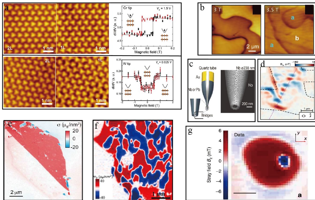
Figure 25. (a) STM images of a CrBr 3 film with adjacent monolayer (1L) and bilayer (2L) regions and spin-polarized tunneling signals on the bilayer regions as a function of magnetic field. Adapted with permission from ref 20. Copyright 2019 AAAS. (b) Antiferromagnetic domain patterns in MnBi 2 Te 4 measured with MFM. Adapted with permission from ref 253. Copyright 2020 American Chemical Society. (c) Schematic illustration of the pulled quartz tube with two Nb or Pb superconducting leads connected to Au electrodes and image of a Nb SQUID-on-tip device. Inset: Magnified view showing the superconducting loop on the apex of the tip. The bridges that reside in the gap regions between the leads form the two weak links of the SQUID. Adapted with permission from ref 254. Copyright 2013 Nature Springer. (d) Gradient magnetometry signal associated with the fully polarized twisted bilayer graphene device. Adapted with permission from ref 255. Copyright 2021 AAAS. (e–g) Magnetic images obtained with scanning NV magnetometry. (e) Magnetization image of bilayer/trilayer CrI 3 adapted with permissions from ref 21. Copyright 2019 AAAS. (f) The magnetic domains in bilayer CrBr 3 adapted with permission under a Creative Commons CC BY license from ref 256. Copyright 2021 Springer Nature. (g) Stray field map of a magnetic skyrmion in the CoFeB system adapted with permission under a Creative Commons CC BY license from ref 257. Copyright 2018 Springer Nature.
