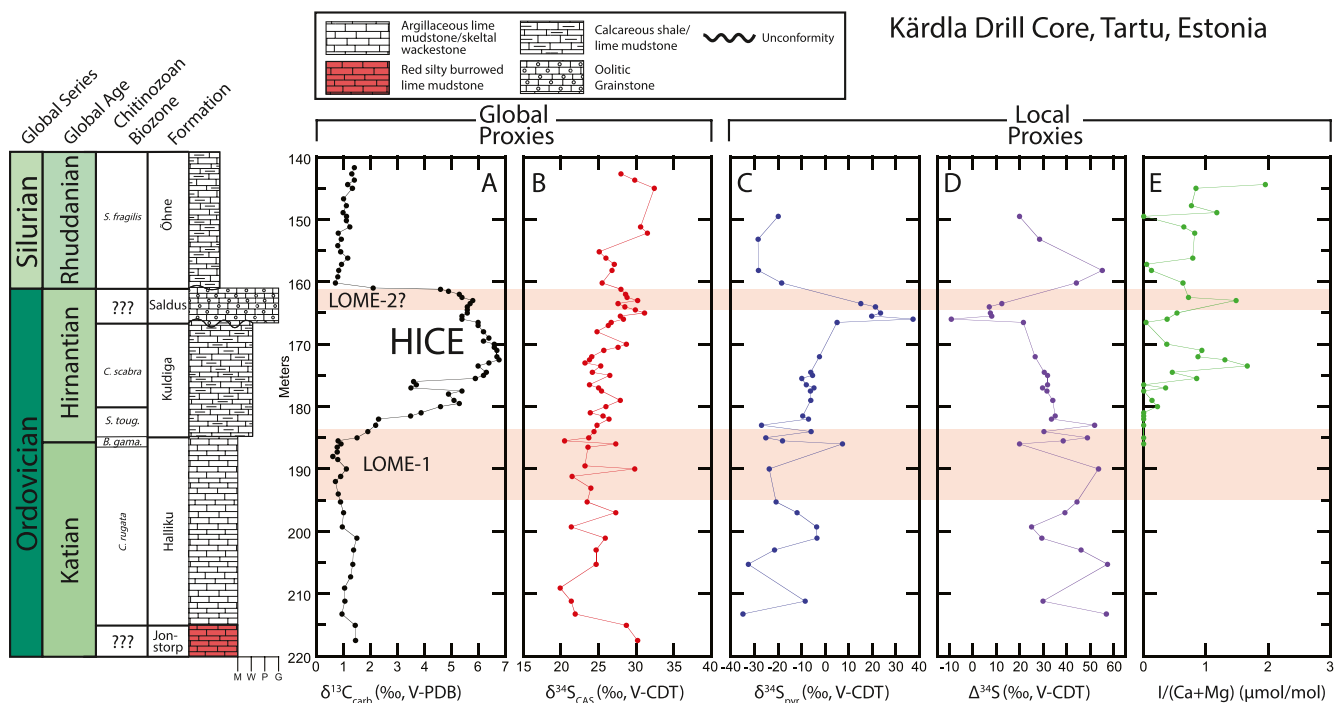
Figure 3. Geochemical and lithologic profile of the Kärđla Drill Core, Estonia. Chitinozoan biozones and lithologies are modified from Brechley et al., 2003 and Young et al., 2010. (a) \delta^{13}\text{C}_{\text{carb}} replotted from Young et al., 2010. (b) \delta^{34}\text{S}_{\text{CAS}} this study. (c) \delta^{34}\text{S}_{\text{pyr}} this study. (d) \Delta^{34}\text{S} , this study. (e) \text{I}/(\text{Ca} + \text{Mg}) ratios, this study.
