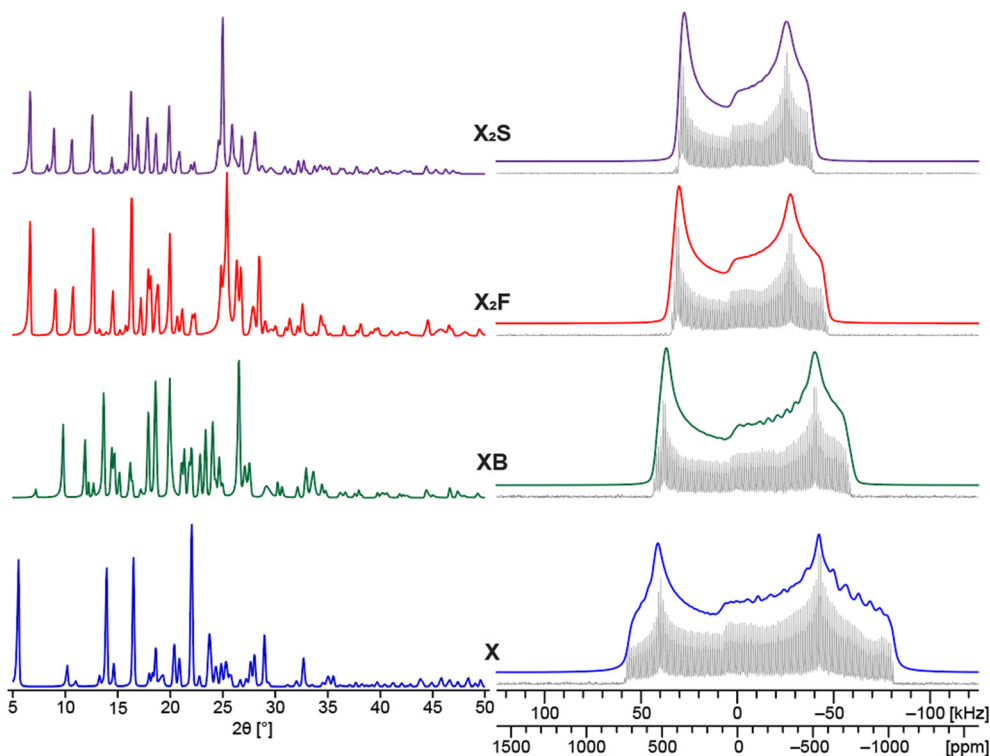
Fig. 1 Experimental PXRD (left) and ^{35}\text{Cl}(^1\text{H}) CPMG SSNMR spectra acquired at B_0 = 18.8 T with simulated fits (right) of X (blue), XB (green), \text{X}_2\text{F} (red), and \text{X}_2\text{S} (purple).
