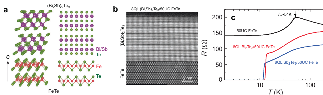
Fig. 1 | Interfacial superconductivity in MBE-grown (Bi, Sb) 2 Te 3 /FeTe heterostructures. a Schematic of the (Bi, Sb) 2 Te 3 /FeTe heterostructure. b Cross-sectional ADF-STEM image of the 8QL (Bi, Sb) 2 Te 3 /50UC FeTe grown on a heat-treated SrTiO 3 (100) substrate. c Temperature dependence of the sheet longitudinal resistance R
