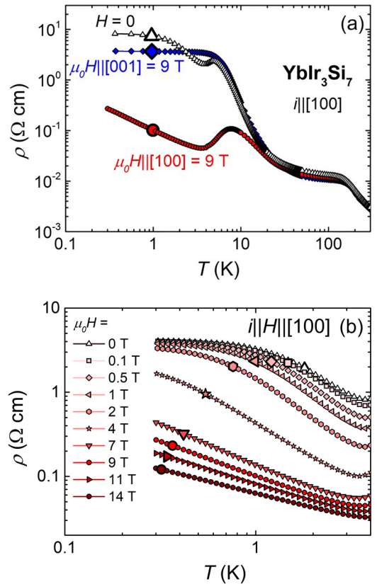
FIG. 7. (a) Log-log plot of the temperature-dependent resistivity in H = 0 (triangles) and in applied magnetic field \mu_0 H = 9 T, H \parallel [100] (circles), and H \parallel [001] (diamonds), and (b) H \parallel [100] from 0 to 14 T.
