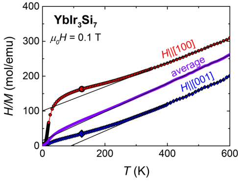
FIG. 10. Anisotropic inverse magnetic susceptibility measurements (symbols) and calculated polycrystalline average H/M_{\text{ave}} (line) with M_{\text{ave}} = 2/3M_{100} + 1/3M_{001} . Solid black lines are linear fits above 350 K, providing evidence of Curie-Weiss behavior.
