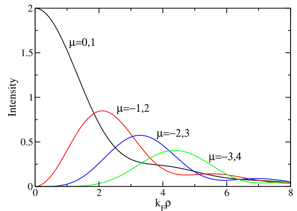
Figure 2. Intensities of the peaks as a function of k_F \rho for several \mu . In general the intensity decreases with \tilde{\rho} and \mu , but not necessarily monotonically.
