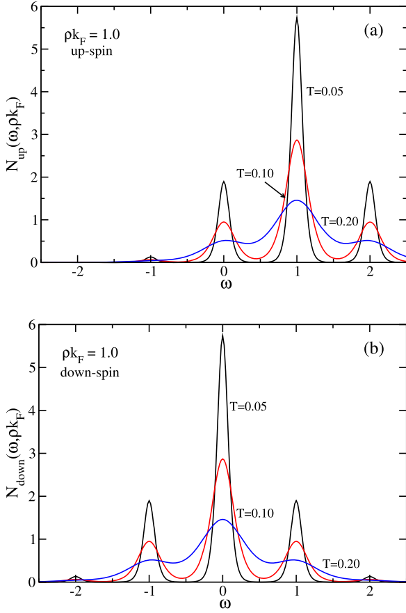
Figure 3. Spin-polarized LDOS (arbitrary units) of the bound states in the vortex as a function of energy \omega for \tilde{\rho} = 1.0 from the center of the core, (a) up-spin and (b) down-spin polarization. The polarization is consequence of the spin-orbit interaction. The three curves in each panel represent the temperatures T = 0.05 (black), T = 0.1 (red) and T = 0.2 (blue). The sum of the up-spin and down-spin LDOS yield the total LDOS shown figure 1(b). Again, K = 0.01\tilde{\rho}^2 and all energies are in units of \Delta_\infty^2/E_F .
