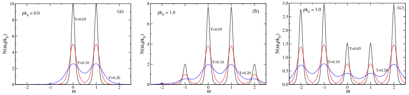
Figure 1. LDOS of the bound states in the vortex as a function of energy \omega for three positions from the center of the core: (a) at the center ( \tilde{\rho} = 0.0 ), (b) at \tilde{\rho} = 1.0 and (c) \tilde{\rho} = 3.0 . The three curves in each panel represent different temperatures: T = 0.05 (black), T = 0.1 (red) and T = 0.2 (blue). Note that the height of the peaks decreases dramatically with T . In the limit T \rightarrow 0 the peaks are delta-functions. We chose K = 0.01\tilde{\rho}^2 . All energies are in units of \Delta_\infty^2/E_F and the LDOS is in arbitrary units but the same for all three panels. Note that the LDOS is not particle–hole symmetric.
