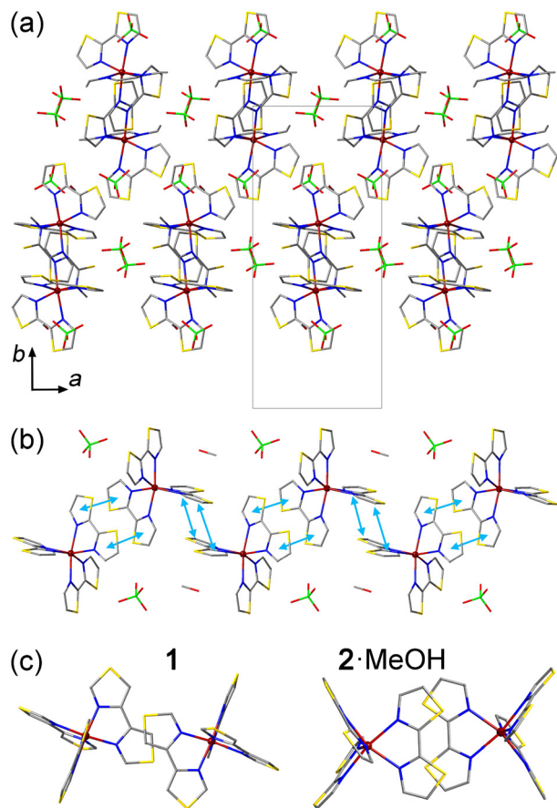
Fig. 2 (a) The crystal packing of 2-MeOH viewed down the c axis to reveal the columns of [\text{Fe}(\text{2bt})_3]^{2+} cations. The unit cell is shown with solid gray lines. The H atoms are omitted for clarity. (b) A side view of a single column of cations, highlighting the \pi - \pi interactions with light-blue double arrows. (c) The top view of \pi - \pi overlaps between the 4bt and 2bt ligands in 1 and 2-MeOH, respectively. Color scheme: Fe = garnet, S = gold, Cl = green, O = red, N = blue, C = gray.
