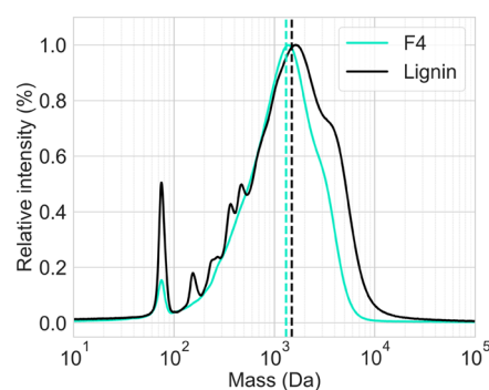
Figure 2. GPC-UV-DAD chromatograms normalized with intensity for BTG BTL fraction F4 and regenerated alkali lignin. The retention time was converted to molecular weights using a calibration curve derived from polystyrene standards.
