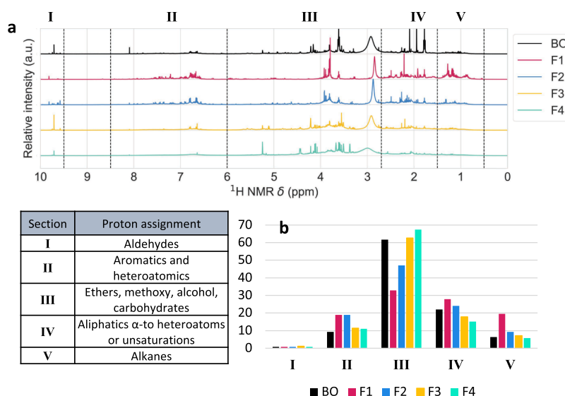
Figure 6. Proton NMR (a) spectra for the samples, after removal of the signals attributed to deuterated acetone 2.04 ppm, and (b) bar chart of relative integration results in the sections of interest.
