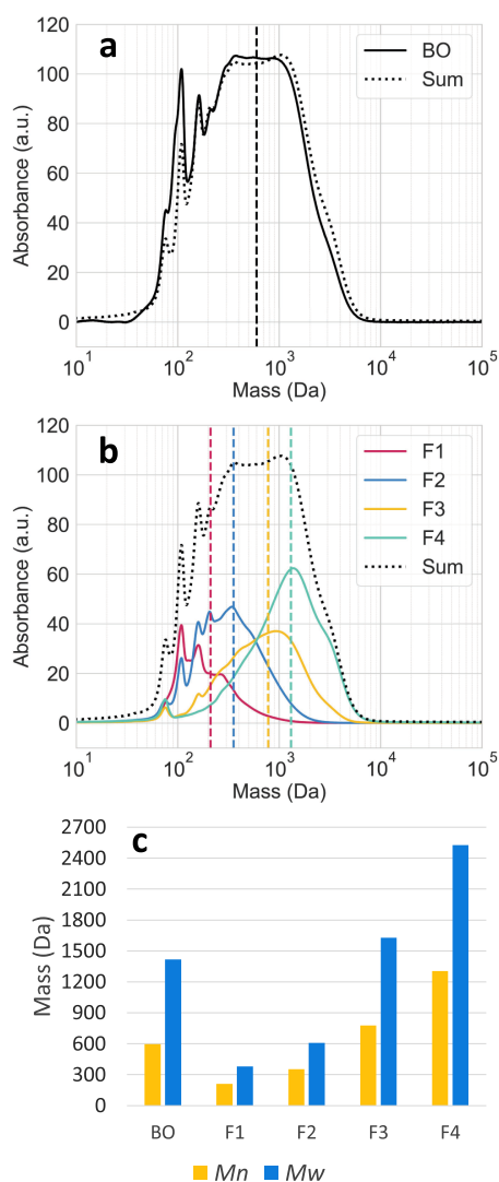
Figure 1. GPC-UV-DAD chromatograms of (a) bio-oil sample (BO) with M_n 597 Da (dotted vertical line). (b) Chromatograms of fractions F1, F2, F3, and F4, each adjusted for gravimetric factors, with their respective M_n values represented by dotted vertical lines at 210, 354, 776, and 1303 Da. The combined reconstructed signal at 254 nm is shown by the 'Sum' line. (c) Bar graph illustrating the values of M_n and M_w of each sample. Retention time converted in molecular weights using a calibration curve derived from polystyrene standards (see original chromatogram Figure S3).
