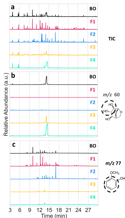
Figure 3. GCMS Chromatograms, the data was normalized using the sample with the highest abundance. (a) TIC, (b) peaks that feature the fragment ion with m/z 60 ( ^+C_2H_4O_2 ), and (c) peaks that reveal the fragment ion with m/z 77 ( ^+C_6H_5 ).
