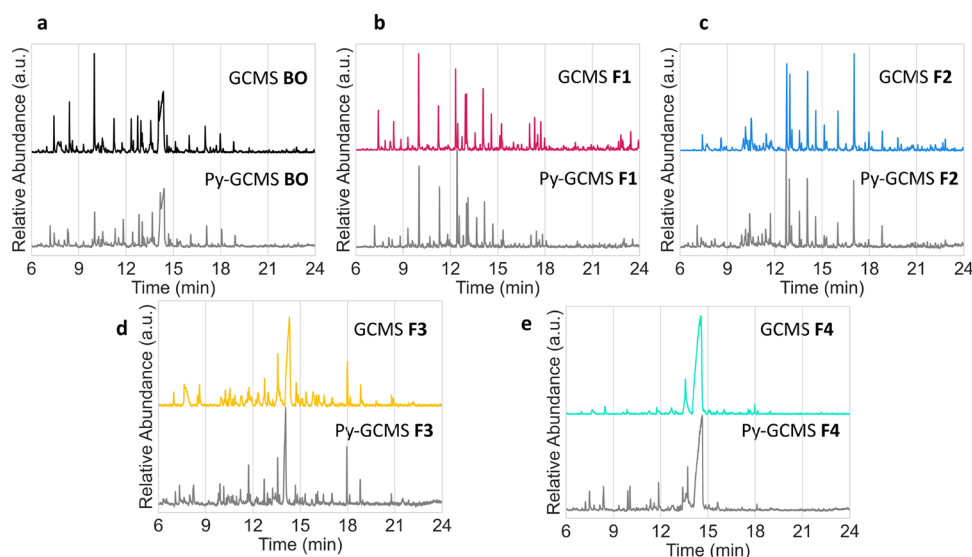
Figure 5. GCMS (shown in different colors) and Py-GCMS (shown in gray) TIC normalized chromatograms for all the samples: (a) whole BO, (b) F1, (c) F2, (d) F3, and (e) F4.
