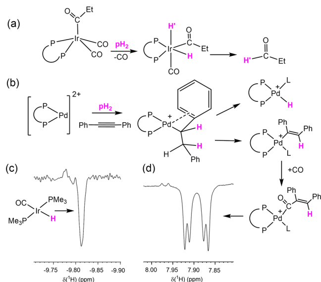
Figure 6. The oneH-PHIP effect has allowed the detection of several single-spin hyperpolarized products. This effect results from the creation of a hyperpolarized AB-type spin system for the p\text{-H}_2 -derived protons (indicated with pink H atoms in (a) and (b)), with subsequent further reaction producing single spin hyperpolarized products. Examples shown here include (a) aldehydes, 158 (b) and (c) metal hydride complexes, 156,157 and (d) vinyl-containing species. 158 The NMR traces illustrate the typical appearance of a single spin-polarized resonance under ^{31}\text{P} decoupling in the case of (c).
