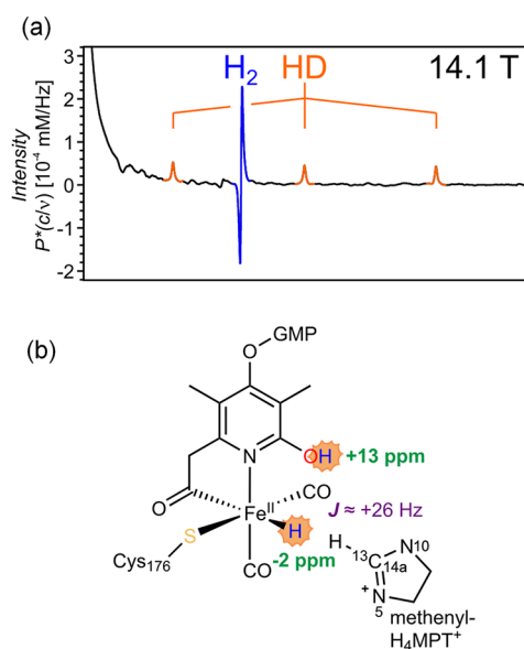
Figure 14. Using PHIP to reveal hitherto unobservable intermediates of [Fe] hydrogenase. (a) Hyperpolarized signals were observed when p\text{H}_2 was supplied to an enzymatic solution of the hydrogenase containing methenyl- \text{H}_4\text{MPT}^+ . A PNL effect and oneH-PHIP hyperpolarized HD signals demonstrate the activation of p\text{H}_2 by hydrogenase. (b) The reaction intermediate was determined using observed NMR parameters and analysis of chemical exchange, and it was derived from a crystal structure quantum mechanical optimization of the structure. Adapted from Kaltschnee et al. 153 Copyright 2024 Springer Nature. This publication is licensed under CC-BY 4.0.
