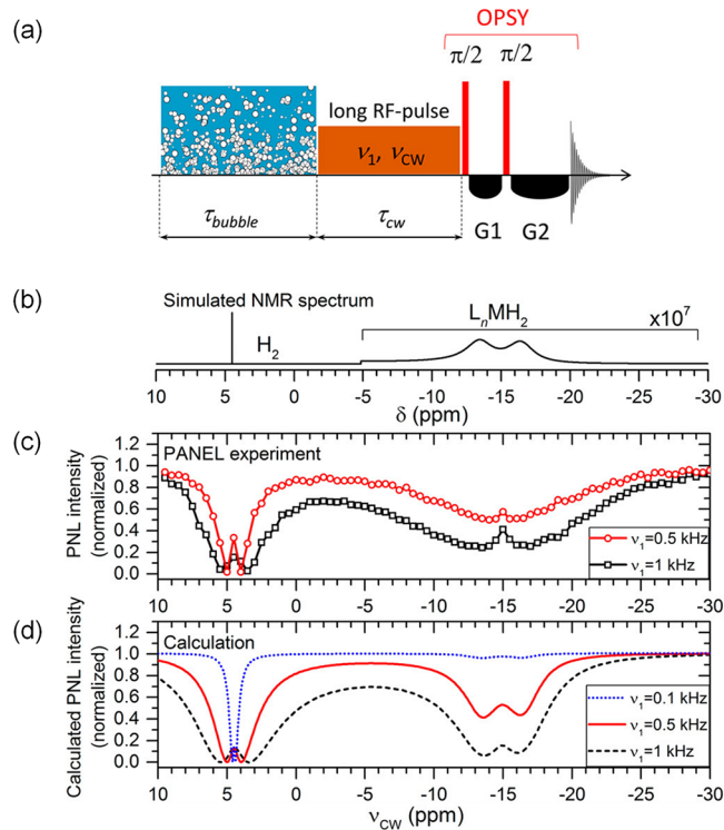
Figure 5. PANEL – A combination of the CEST method and the PNL effect boosts the sensitivity of catalytic intermediate detection. (a) Scheme of the PANEL (partially negative line) experiment for indirectly detecting the hidden hydrogen catalyst complex ( L_nMH_2 ). (b) Calculated NMR spectrum of the hidden complex, magnified by a factor of 10^7 . (c) Experimental and (d) simulated PANEL spectra showing the signal of the hidden complex (lines at –16.5 ppm and –13.5 ppm). Adapted with permission from Kiryutin et al. 132 Copyright 2017 American Chemical Society.
