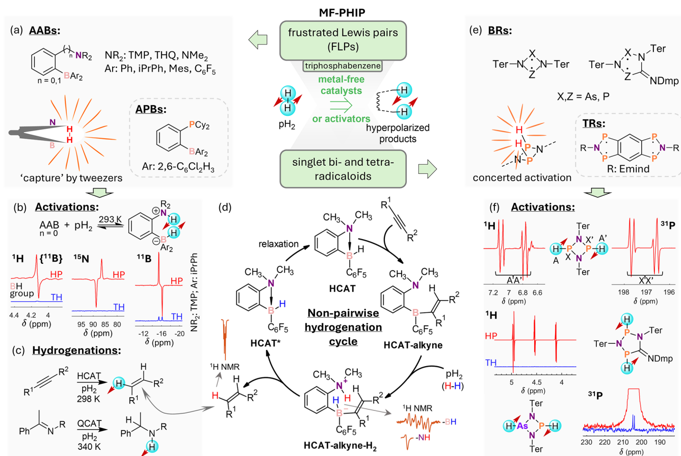
Figure 9. An overview of metal-free PHIP (MF-PHIP). The central top part highlights that MF-PHIP effects have been demonstrated in activation of pH_2 using frustrated Lewis pairs (FLPs) and using bi- and tetra-radicaloids (BRs and TRs). Correspondingly, the structures of ansa -aminoborane (AAB) and ansa -phosphinoborane (APB) FLPs are presented in (a). AABs are referred to as molecular tweezers for pH_2 . pH_2 activation under ambient conditions using ortho -phenylene AABs ( n = 0 ) accompanied by the corresponding hyperpolarized NMR spectra is illustrated in (b). See (a) for the definition of n . In addition to ^1H , ^{15}N and ^{11}B nuclei are also hyperpolarized spontaneously at high magnetic fields in this process. Alkyne and imine hydrogenation reactions catalyzed by AABs HCAT ( n = 0 ; NR_2 = NMe_2 ; Ar = C_6F_5 ; R' = H ) and QCAT ( n = 1 ; NR_2 = THQ ; Ar = C_6F_5 ), respectively, are shown in (c). Additionally, the catalytic cycle of alkyne hydrogenation using the HCAT AAB catalyst is presented in (d). Typical ^1H NMR signals of the reaction intermediate and the reaction product are shown next to the corresponding structures in the cycle. Structures of BR and TR molecules that demonstrated hyperpolarization effects in pH_2 activations are depicted in (e). Corresponding examples of enhanced ^1H and ^{31}P NMR signals observed in reactions with BR molecules are shown in (f). The structures of the corresponding BR- H_2 adducts are depicted next to the spectra. Abbreviations: TMP = N-2,2,6,6-tetramethylpiperidiny; THQ = N-tetrahydroquinolinyl; iPrPh = 2-isopropylphenyl; Mes = mesityl; Cy = cyclohexyl; Ter = 2,6-dimesitylphenyl; Dmp = 2,6-dimethylphenyl; Emind = 1,1,7,7-tetraethyl-3,3,5,5-tetramethyl-s-hydrindacenyl. (d) Adapted from Zakharov et al. 150 Copyright 2022 John Wiley and Sons. This publication is licensed under CC-BY 3.0.
