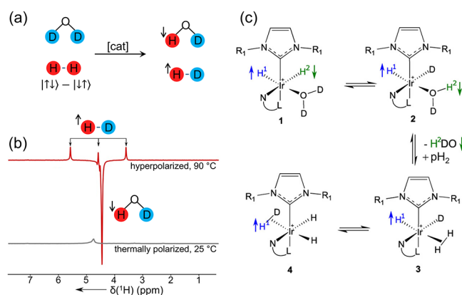
Figure 7. (a) H/D exchange, in the presence of a water-soluble iridium catalyst and histidine, leading to hyperpolarization of HD and HDO and (b) the resulting NMR spectrum, in comparison to the thermally polarized spectrum. (c) The proposed “NEPTUN” mechanism underpins the spectrum. (a, b) Adapted with permission from Lehmkuhl et al. 170 Copyright 2017 John Wiley and Sons. (c) Adapted with permission from Emondts et al. 110 Copyright 2018 John Wiley and Sons.
