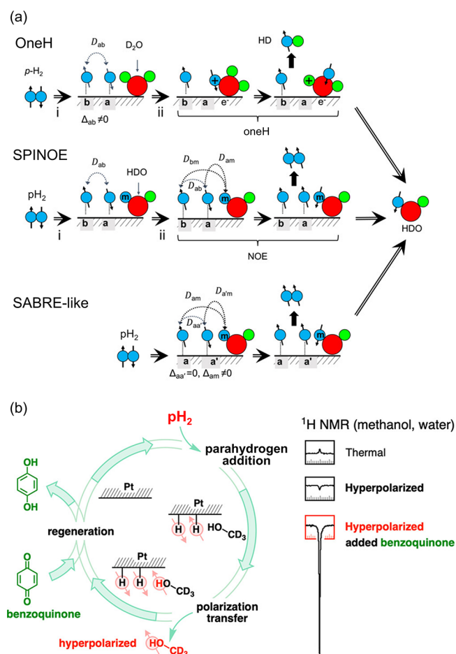
Figure 8. (a) Possible mechanisms underpinning surface-mediated hyperpolarization of liquid water. (b) Mechanism of benzoquinone scavenging of depolarized H adatoms on Pt/C, and its effect on the SWAMP signals. (a) Adapted with permission from Zhao et al. 155 Copyright 2018 Elsevier. (b) Reproduced from Norcott. 180 Copyright 2023 American Chemical Society. This publication is licensed under CC-BY-NC-ND 4.0.
