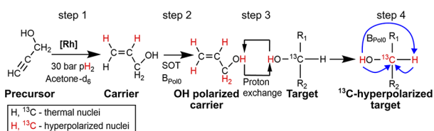
Figure 11. Schematic view of parahydrogen-induced polarization by chemical exchange (PHIP-X). PHIP-X consists of four essential steps: hydrogenation of the carrier agent (step 1), the polarization of the exchanging protons (step 2), transfer of the exchanging protons from the carrier to the target molecule (step 3), and polarization of the target nucleus (step 4) using RF-induced spin order transfer technique or free evolution at low and ultralow magnetic fields. Adapted from Them et al. 222 Copyright 2024 Springer Nature. This publication is licensed under CC BY 4.0.
