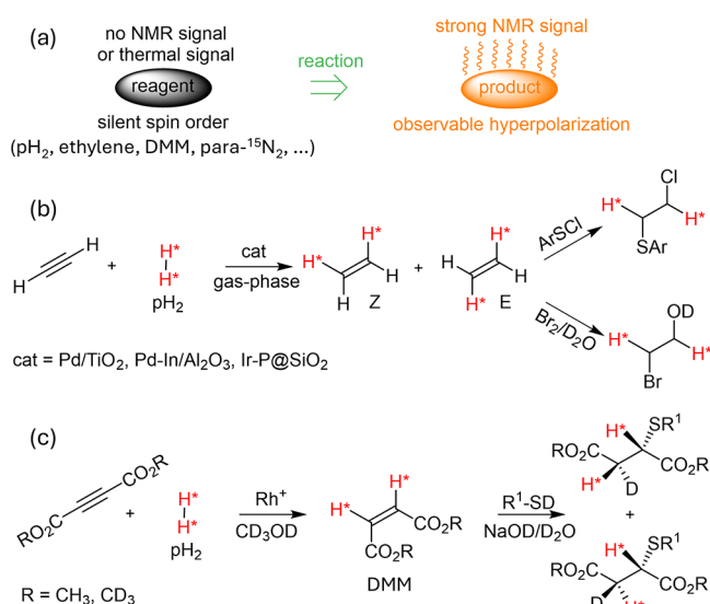
Figure 10. (a) A general scheme of formation of compounds with hyperpolarized spins in chemical reactions of symmetric molecules, such as pH 2 , ethylene, DMM, and para- 15 N 2 , accommodating otherwise unobservable nuclear spin orders. (b) The chemical synthesis of Z - and E -ethylene from acetylene and pH 2 over various heterogeneous catalysts, as well as subsequent reactions revealing hyperpolarization. (c) The chemical synthesis of dimethyl maleate (DMM) molecules in hydrogenation with pH 2 over a cationic Rh + catalyst, followed by their subsequent reaction with thiol molecules to reveal hyperpolarization. Abbreviations: DMM - dimethyl maleate.
