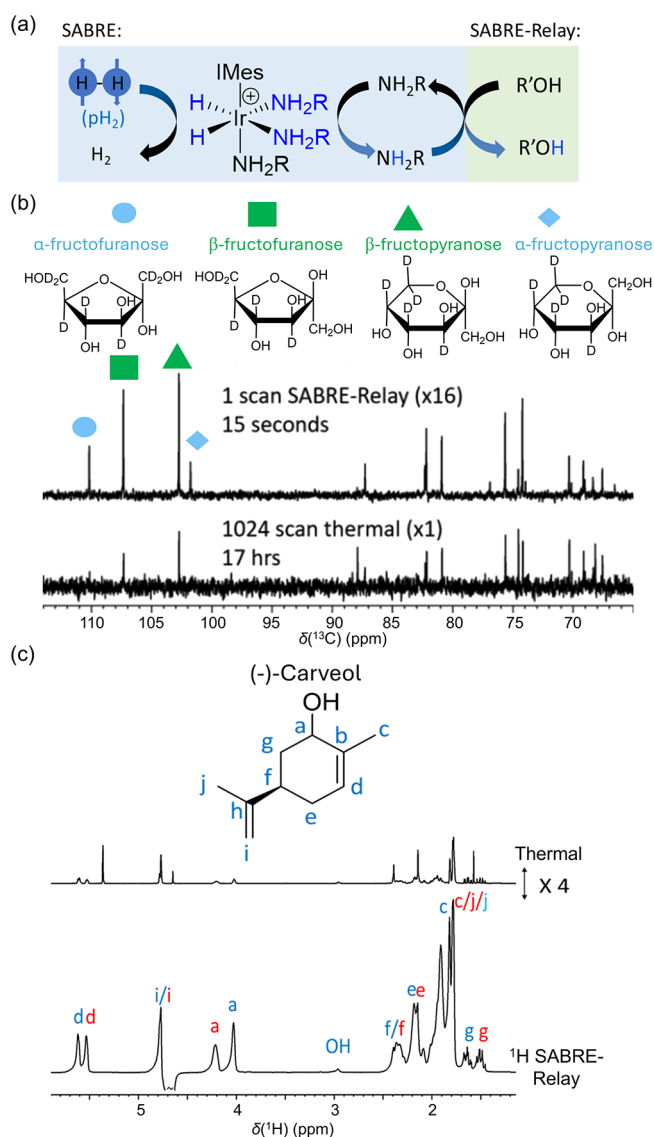
Figure 12. Demonstration of the SABRE-Relay effect. (a) Depiction of the SABRE-Relay method. (b) SABRE-Relay can allow quantification of isomer ratios of fructose in a single scan ^{13}\text{C} measurement or (c) quantification of diastereomer ratios of the natural product (–)-carveol from a single scan ^1\text{H} measurement. Details for (b): ^{13}\text{C}\{^1\text{H}\} NMR spectra (right) acquired for 40 mM of D-fructose (natural ^{13}\text{C} abundance) with 23.8 mM benzyl- d_7 -amine and 4.8 mM of [\text{Ir}(\text{Cl})(\text{COD})(\text{SIMes-}d_{22})] (where COD is cis,cis -cyclooctadiene and SIMes is 1,3-bis(2,4,6-trimethylphenyl)-4,5-dihydroimidazol-2-ylidene) in a 0.65 mL \text{DCM-}d_2 :DMF (1.6:1) mixture measured at 9.4 T. The bottom spectrum shows the result of a thermally polarized signal averaging over 1024 scans (approximately 17 h), and the middle spectrum represents the single scan SABRE-Relay hyperpolarization measurement recorded after shaking the sample with \text{pH}_2 at 6.5 mT. Details for (c): Exemplar single scan thermally polarized (above) and ^1\text{H} SABRE-Relay hyperpolarized (lower) ^1\text{H} NMR spectra for a sample of [\text{Ir}(\text{Cl})(\text{COD})(\text{IMes})] (5 mM), \text{NH}_3 (30 mM), (–)-carveol (25 mM) and \text{pH}_2 (3 bar) in \text{DCM-}d_2 (0.6 mL). The resonance labels in red and blue correspond to the two diastereomers. The hyperpolarized NMR spectrum is recorded immediately after shaking the sample for 10 s with fresh \text{pH}_2 at 6.5 mT. (a, c) Adapted from Alshehri et al. 228 Copyright 2023 Royal Society of Chemistry. This publication is licensed under CC BY 3.0. (b) Adapted from Richardson et al. 226 Copyright 2019 Royal Society of Chemistry. This publication is licensed under CC BY 3.0.
