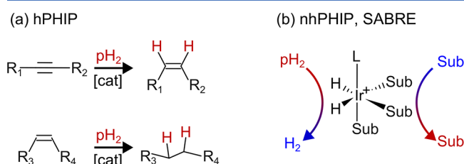
Figure 1. hPHIP and SABRE. Schematics of (a) hPHIP, whereby parahydrogen ( pH_2 ) is added to an unsaturated bond in the presence of a catalyst, [cat], and (b) SABRE, where a ligating substrate, Sub, and pH_2 undergo reversible exchange at a catalyst. The typical SABRE auxiliary ligand L is IMes = 1,3-bis(2,4,6-trimethylphenyl)-1,3-dihydro-2H-imidazol-2-ylidene.
