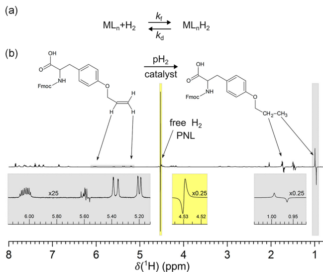
Figure 4. Partial Negative Line effect induced by a catalyst–pH 2 interaction. (a) Chemical exchange of pH 2 with the metal center ML_n of the catalyst results in the PNL effect on free H 2 . (b) ^1H PHIP NMR spectrum recorded during the hydrogenation of Fmoc-O-allyl-tyrosine (left) to Fmoc-O-propyl-tyrosine (right) with pH 2 , showing a strong PNL signal for free H 2 at 4.53 ppm. Adapted with permission from Kiryutin et al. 132 Copyright 2017 American Chemical Society.
