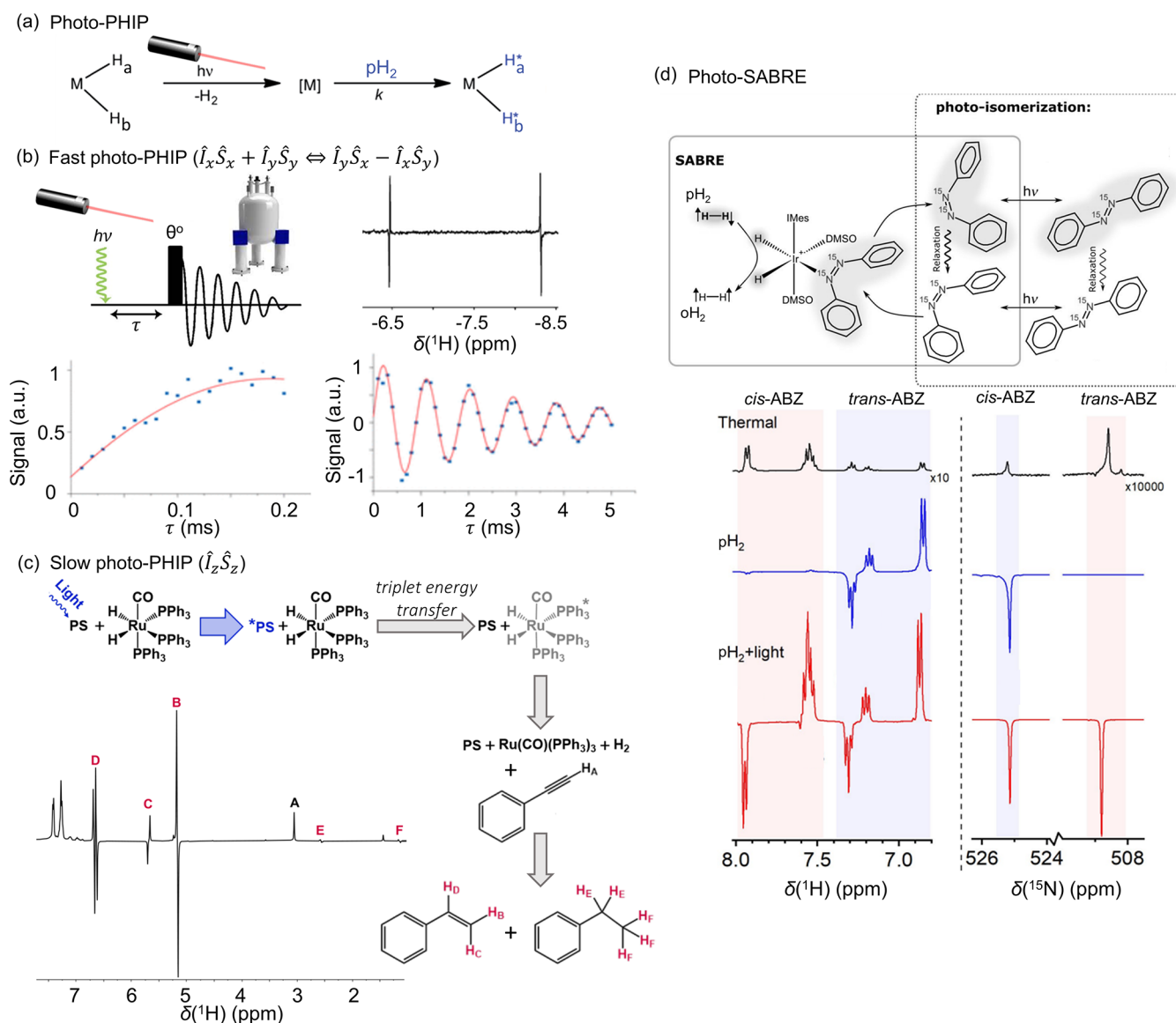
Figure 3. Examples of photo-PHIP. (a) The outline of a photo-PHIP experiment in which light-induced ligand dissociation creates a metal complex [M] that can add pH_2 to create an inequivalent metal dihydride species with PHIP-enhanced hydride NMR signals. (b) Depiction of laser-pump NMR-probe spectroscopy in which laser irradiation stimulated H_2 - pH_2 exchange followed by NMR detection (where \theta is typically 45^\circ or 90^\circ ), with a variable delay between the two (top left). The NMR spectrum at the top right is a single-laser shot, single 90^\circ RF pulse, pH_2 -enhanced ^1H\{^{31}P\} NMR spectrum of the hydride region of [Ru(PPh_3)_3(CO)(H)_2] with \tau = 0.05 ms (broadband ^{31}P decoupling). When the delay is on the millisecond time scale, the zero quantum coherences of pH_2 in the chemically inequivalent dihydride complex can evolve due to the chemical shift difference from unobservable \hat{I}_x\hat{S}_x + \hat{I}_y\hat{S}_y to observable \hat{I}_y\hat{S}_x - \hat{I}_x\hat{S}_y . The lower kinetic traces show the hydride signal integral at \delta \sim -6.5 ppm from ^1H\{^{31}P\} NMR spectra of [Ru(PPh_3)_3(CO)(H)_2] ( 1 \times 10^{-3} M, 3 bar pH_2 ) as a function of \tau . Experimental points are shown in blue with fitted red lines. This spin evolution can give information about kinetic hydrogen addition rates. (c) Slow photo-PHIP leading to hyperpolarized styrene and ethylbenzene after [Ru(H)_2(PPh_3)_3(CO)] and an iridium photosensitizer (PS) are irradiated at 420 nm in DCM- d_2 at 298 K. 128 In these cases, delays between laser irradiation and NMR pulse acquisition are on the order of seconds. Consequently, ZQC coherences are not observed, which is similar to the traditional PASADENA effect. (d) Depiction of photo-SABRE in which a SABRE-catalyst hyperpolarizes cis -azobenzene (ABZ) followed by light irradiation to switch between cis and trans isomers of ABZ (upper). Hyperpolarized molecules are shown with a gray background. 129 Example ^1H (lower left) and ^{15}N (lower right) NMR spectra were recorded after 10 min of light irradiation of a sample containing 56 mM of ^{15}N_2 -ABZ in CD_3OD with 1 mM of [IrCl(COD)(IMes)] and 200 mM DMSO- d_6 at 9.4 T. SABRE polarization transfer to ^1H was performed at 200 nT and that to ^{15}N , at 400 nT. Signals for cis -ABZ are shown with a red background, with those of trans -ABZ with a blue background. (a) Adapted with permission from Procacci et al. 115 Copyright 2016 Royal Society of Chemistry. This publication is licensed under CC BY-NC 3.0. (b) Adapted from Torres et al. 114 Copyright 2014 American Chemical Society. This publication is licensed under CC-BY. (c) Adapted from Brown et al. 128 Copyright 2022 American Chemical Society. This publication is licensed under CC-BY 4.0. (d) Adapted with permission from Kiryutin et al. 129 Copyright 2024 John Wiley and Sons.
