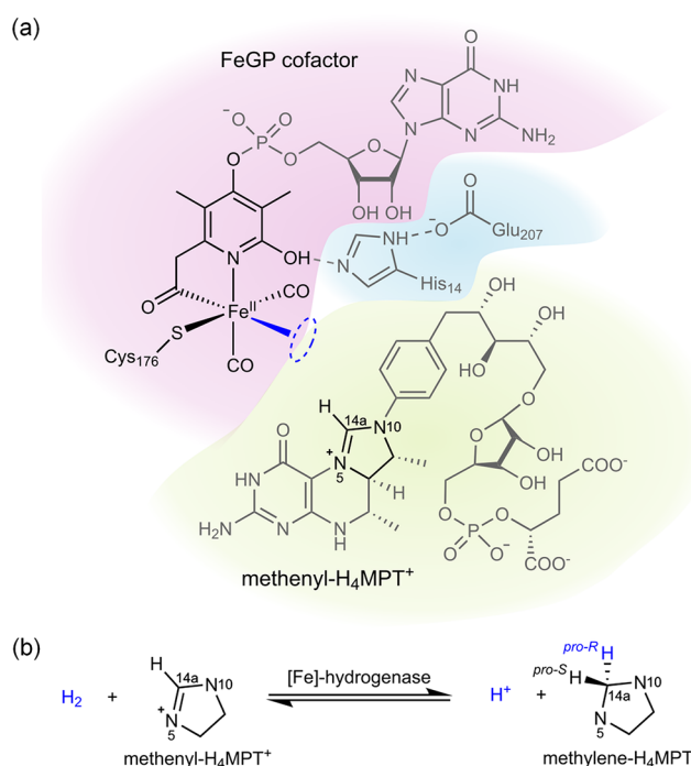
Figure 13. Active site of the mono iron hydrogenase and the hydrogenation reaction. (a) The active site of the [Fe]-hydrogenase, including the iron guanylyl pyridinol and methenyl- H_4MPT^+ . (b) Hydride transfer to the Hpro-R position of the substrate forming methylene- H_4MPT . Adapted from Kaltschnee et al. 153 Copyright 2024 Springer Nature. This publication is licensed under CC-BY 4.0.
