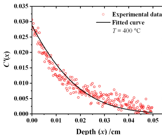
Fig. 9. Normalized ^{16}\text{OD}^- fraction ( C'(x) ) in BCFZY4411 annealed at 400 °C. Red circles refer to experimental data and black line is the fit to Eq. S26. (For interpretation of the references to colour in this figure legend, the reader is referred to the web version of this article.)
