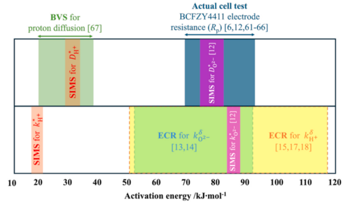
Fig. 11. Comparison of E_a values obtained by BCFZY4411 proton and oxygen kinetic studies through various characterization methods [6,12–15,17,18,61–66] and a theory study [67]. BVS: Bond valence sum analysis, and ECR: Electrical conductivity relaxation.
