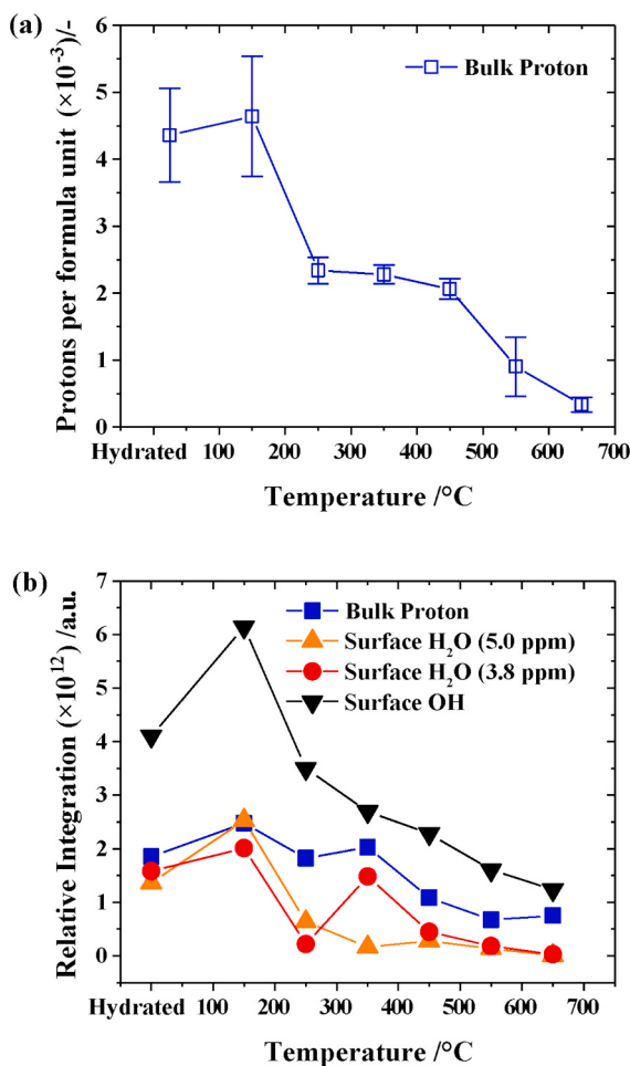
Fig. 8. Examining proton loss in BCFZY4411 using ^1\text{H} solid-state MAS NMR when dehydrated at 150 to 650 °C under dry air. (a) Bulk proton concentrations are determined via an internal standard, adamantane. (b) Relative NMR resonance areal integrals of separate species in BCFZY4411 to determine hydrogen rate loss for each species.
