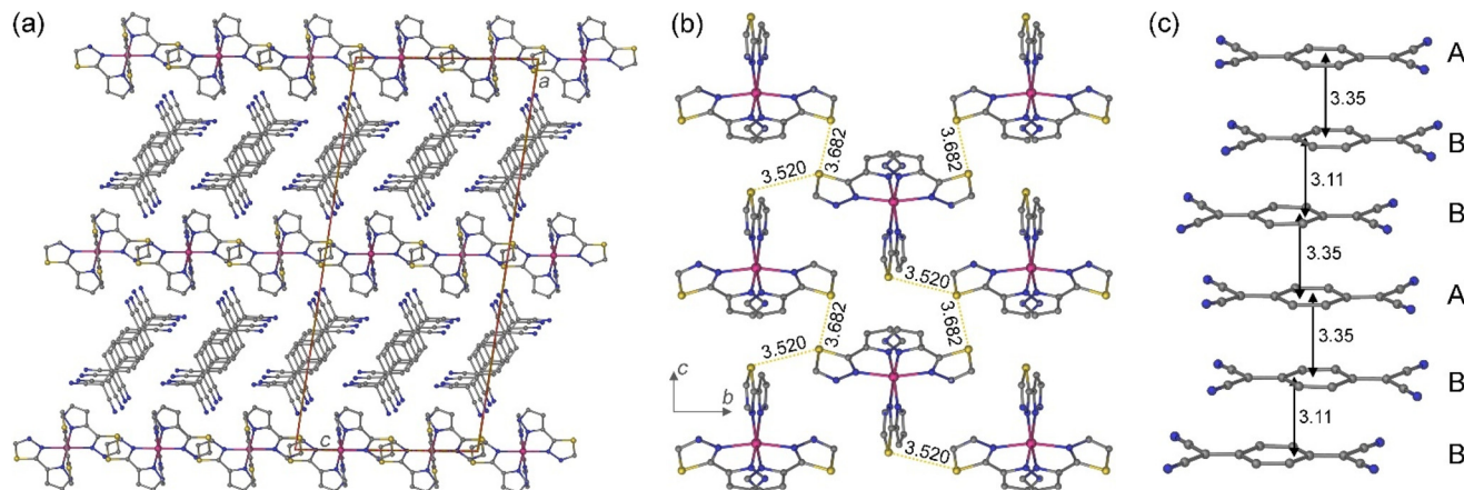
Fig. 2 (a) The crystal packing of 1 viewed parallel to the ac plane, with the columns of the \text{TCNQ}^{\bullet\delta-} anions propagating perpendicular to the plane of the drawing; the unit cell is shown with solid orange lines. (b) A view of a single layer of the [\text{Fe}(\text{3tpH})_3]^{2+} cations in the bc plane; the network of intermolecular \text{S}\cdots\text{S} contacts is shown with dotted yellow lines, with the interatomic distances in Å. (c) The stacking of the \text{TCNQ}^{\bullet\delta-} anions, with the interplanar distances shown in Å. Color scheme: Fe = magenta, S = yellow, N = blue, C = gray. The H atoms are omitted for clarity. Only one part of the disorder is shown for each crystallographically disordered fragment.
