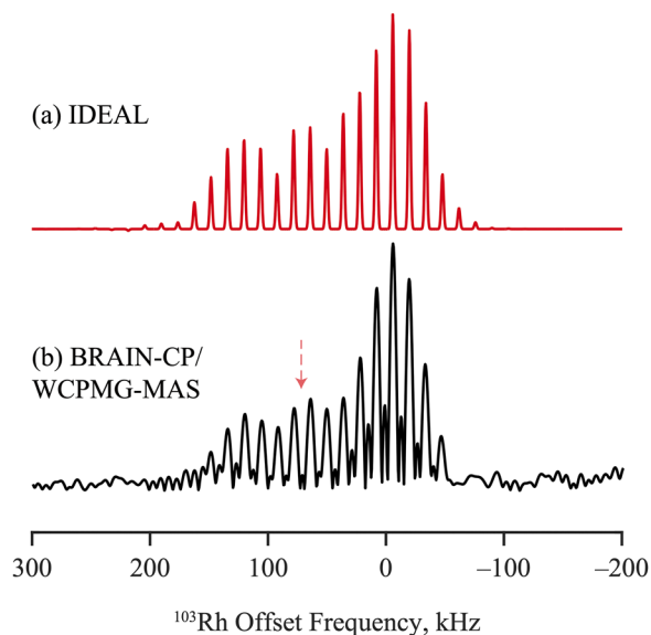
Fig. 9 (a) Simulated and (b) experimental ^{103}\text{Rh} MAS NMR spectra of \text{Rh}_2\text{Cl}_2(\text{COD})_2 acquired at 21.08 T using BRAIN-CP/WCPMG-MAS with \nu_{1,S} = \Delta = \nu_{\text{rot}} = 14 kHz, \tau_{\text{CT}} = 20 ms, and \nu_{1,I} = 35 kHz. The value of \Omega_S/2\pi is indicated by the dotted red arrow. 4096 transients were collected using a recycle delay of 2 s for a total time of ca. 2.3 hours.
