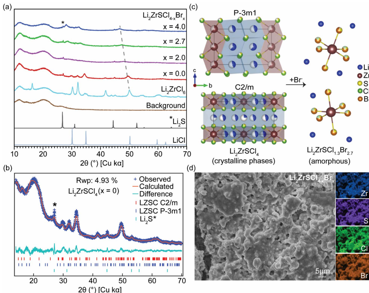
Fig. 1 Structural evolution and morphology of \text{Li}_2\text{ZrSCL}_{4-x}\text{Br}_x ( 0 \leq x \leq 4 ) (a) powder X-ray diffraction of \text{Li}_2\text{ZrSCL}_{4-x}\text{Br}_x showing progressive peak shifts (dashed line), peak broadening, and intensity loss with increasing \text{Br}^- content. (b) Rietveld refinement of \text{Li}_2\text{ZrSCL}_4 ( x = 0 ), confirming a biphasic structure comprising trigonal P\bar{3}m1 and monoclinic C2/m phases. (c) Crystal structure models of the P\bar{3}m1 and C2/m polymorphs of \text{Li}_2\text{ZrSCL}_4 and schematic representation of the structural evolution upon \text{Br}^- substitution, leading to an amorphous \text{Li}_2\text{ZrSCL}_{1.3}\text{Br}_{2.7} network (d) SEM micrograph and corresponding EDS elemental maps showing uniform distribution of Zr, S, Cl, and Br in \text{Li}_2\text{ZrSCL}_{1.3}\text{Br}_{2.7} .
