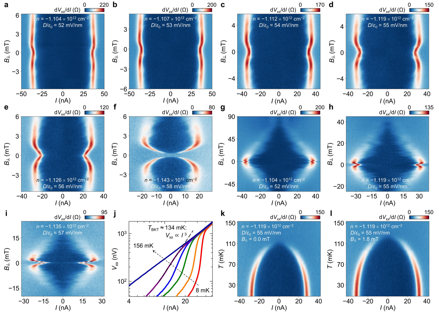
Extended Data Fig. 7 | T - and B_{\perp} -dependent measurements on SC3 in Device R5G-1. a-f , Differential resistance as a function of I and B_{\perp} at different (n, D) points. The enhancement of SC3 by B_{\perp} is observed globally across its phase space. g-i , Differential resistance as a function of I and B_{\perp} at different (n, D) points for a wider range of the magnetic field. Fraunhofer-like patterns arising from quantum interference are observed in i which is adjacent to the phase boundary of SC3, and they become fainter as D/\epsilon_0 decreases. j , V_{xx} versus current I at T = 8 ,
