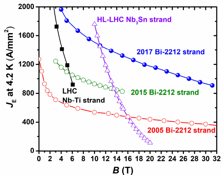
Figure 1. The J_E(B) of the large hadron collider (LHC) insertion quadrupole Cu/Nb-Ti strand (diameter = 0.479 mm, Cu/Nb-Ti = 1.678), the high luminosity (HL)-LHC upgrade QXF RRP® Nb 3 Sn strand (diameter = 0.85 mm, Cu/non-Cu = 1.20 \pm 0.1 ), and three Bi-2212 wires (Ag:AgMg:Bi-2212 \approx 2:1:1), best
