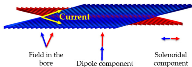
Figure 6. Two-layer CCT concept for dipole magnets.
