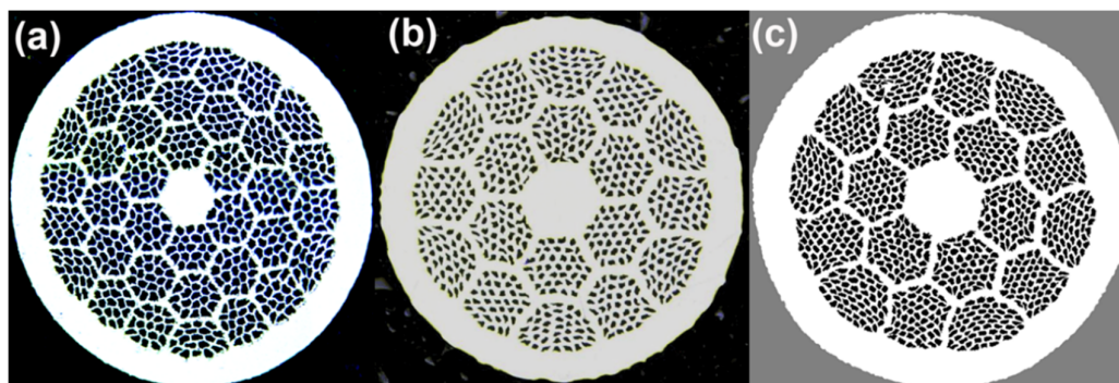
Figure 4. (a) RC1 wire PMM130411, 19 \times 36 architecture, Nexans powder #77; (b) RC2 and RC3 wire PMM101111, 36 \times 18 architecture, Nexans powder #77; (c) RC5 and RC6 wire PMM170123, 55 \times 18 architecture, nGimat powder LXB-52. The photograph of PMM170123 is a courtesy of J. Jiang of NHMFL.
